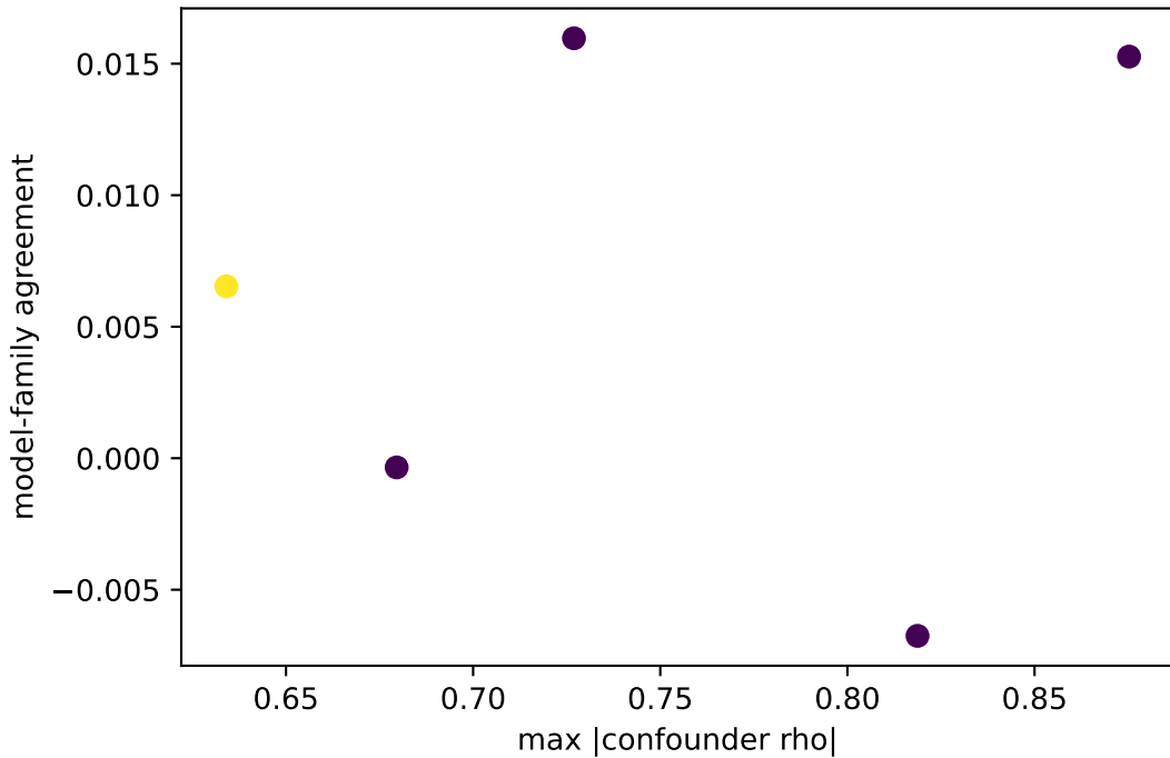
Confounder and agreement screen
