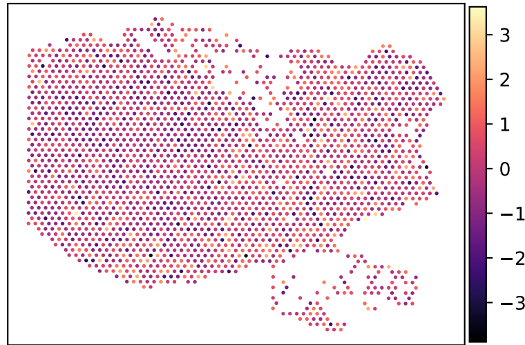
RAF/MAPK target-output z
