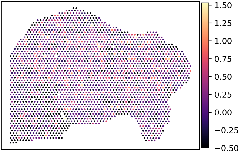
DUSP6 expression z
