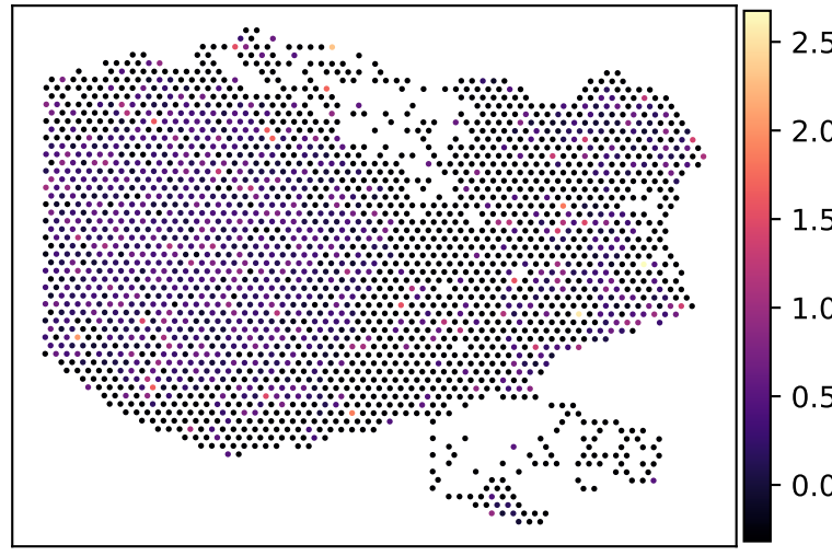
DUSP6 expression z
