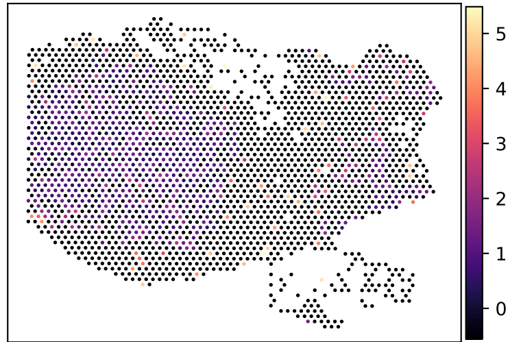
DUSP6 expression z
