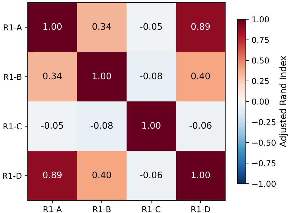
Pairwise ARI between leak-free cluster variants (R1-A,B,D agree; R1-C is immune-axis-only)
