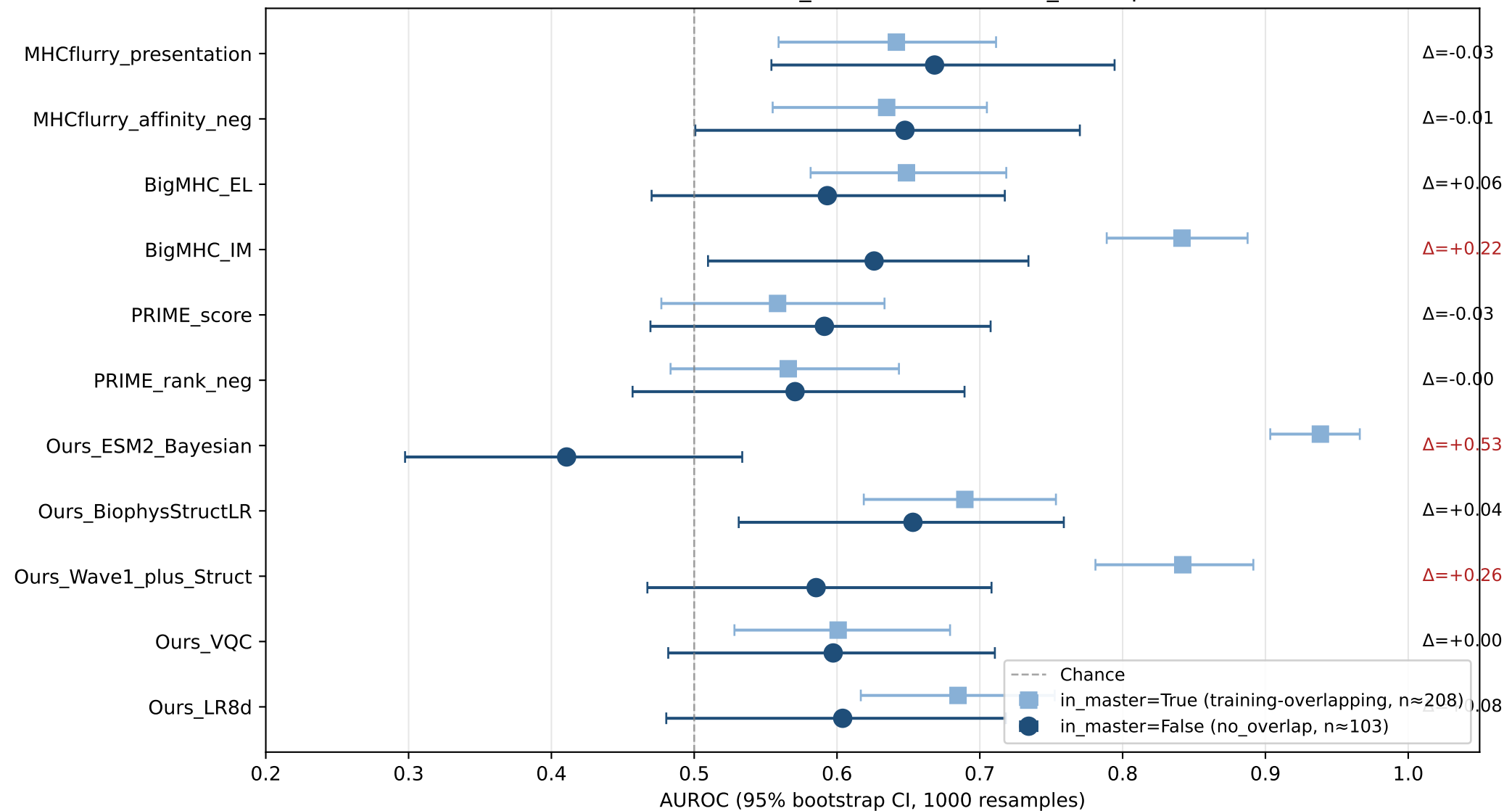
Wave 3 — Leakage Inflation in Neoantigen Immunogenicity Predictors (ITSNdb combined; \Delta = in_master AUROC – no_overlap AUROC)
