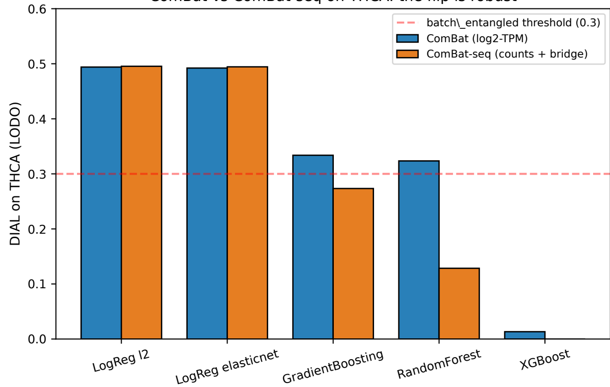
ComBat vs ComBat-seq on THCA: the flip is robust
