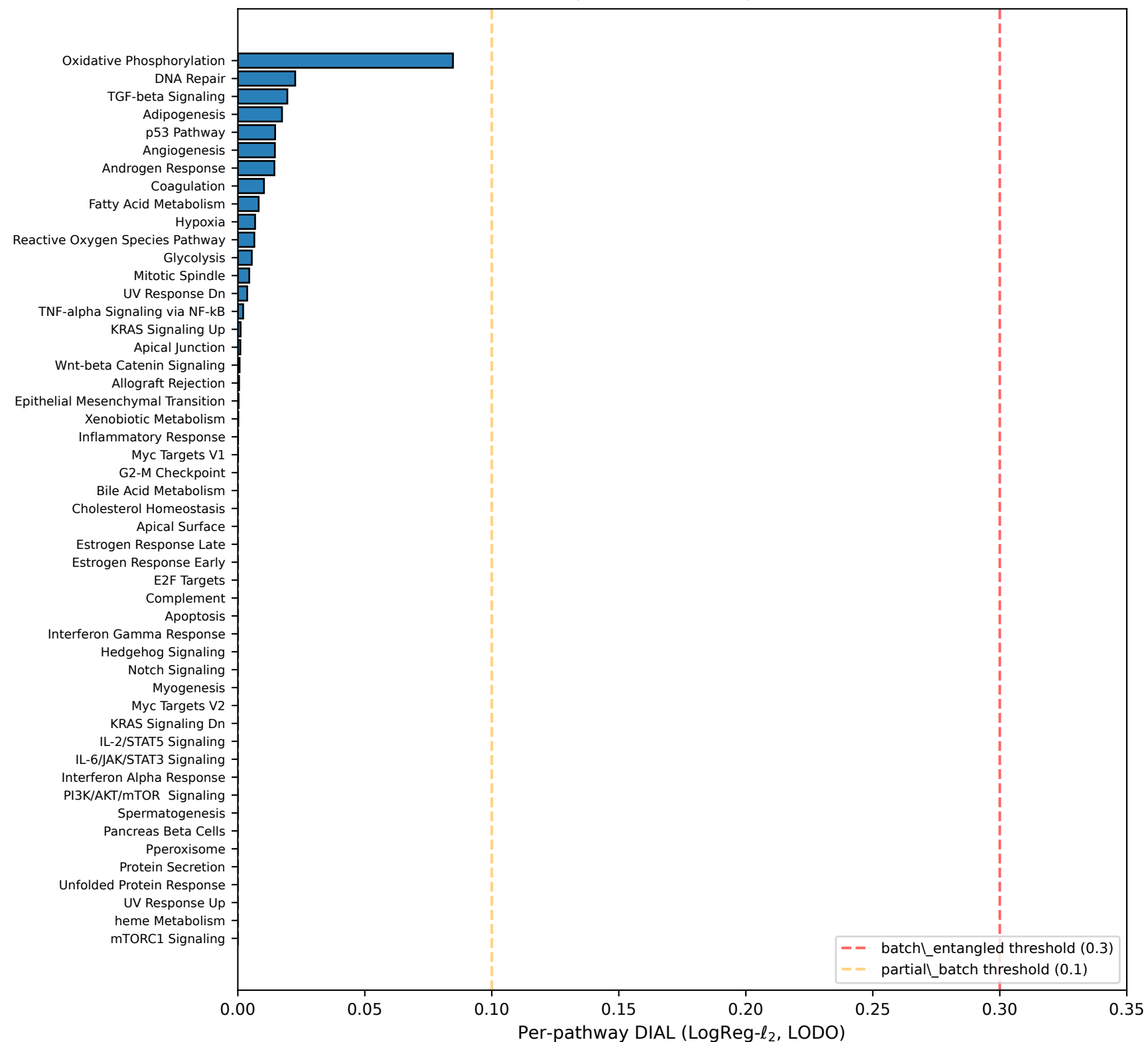
Per-pathway DIAL on 50 MSigDB Hallmark sets (real) max DIAL = 0.085, median = 0.000, 0/50 above threshold
