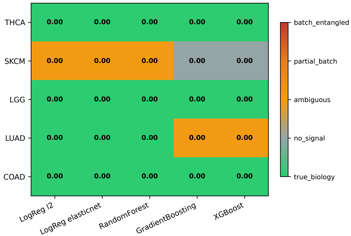
(b) Per-fold — ComBat fit inside each LODO fold (v5.2)
