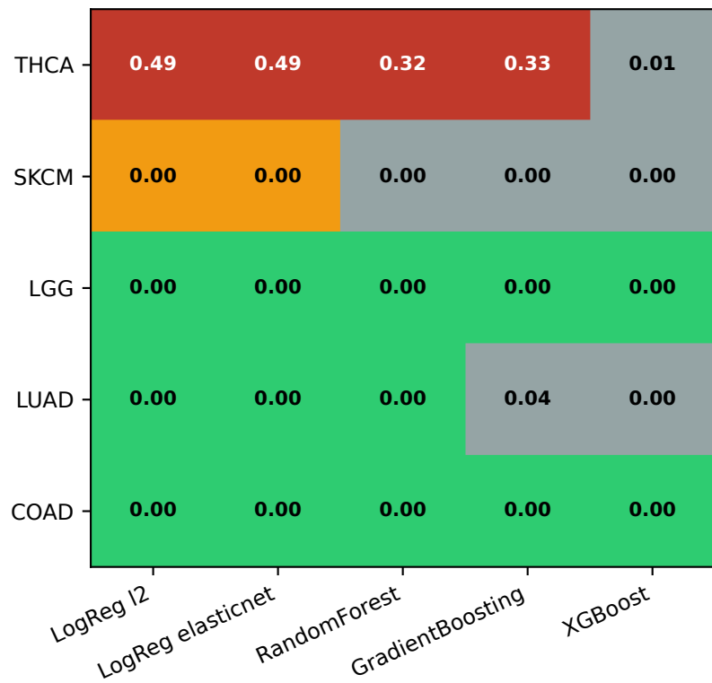
(a) Leaky — ComBat fit on pooled X before LODO (v5.1)
