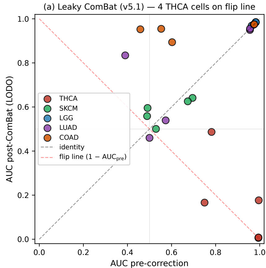
Figure 2. AUC pre vs post — same 25 cells, two protocols
