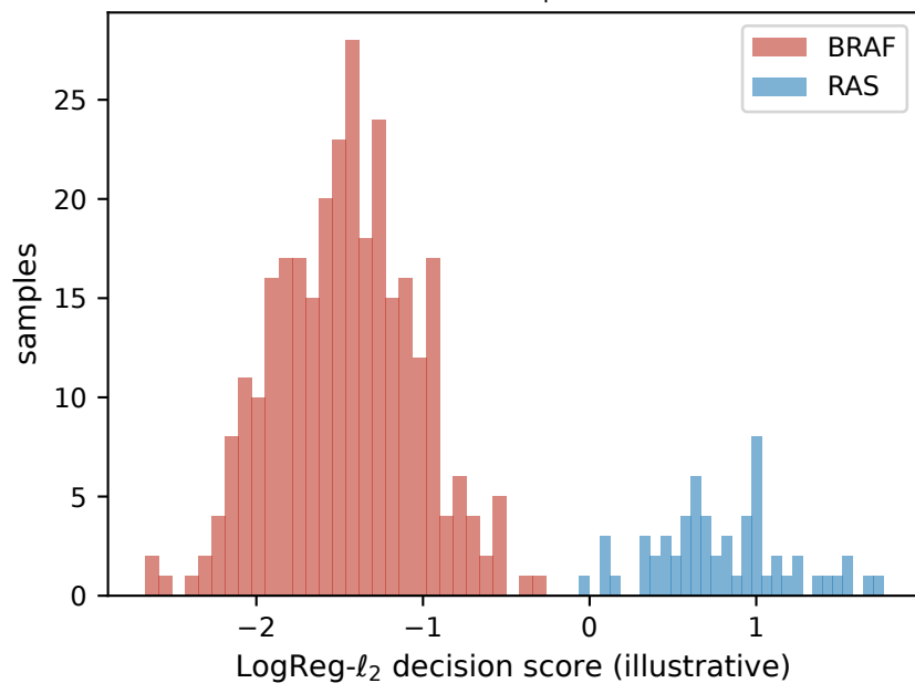
(B) Post-ComBat score (schematic) observed AUC_{post}=0.006
