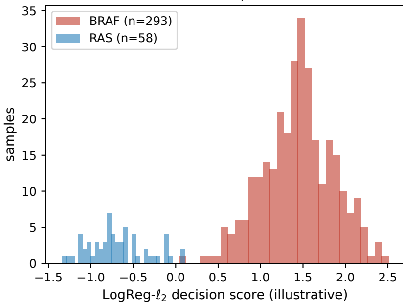
(A) Pre-ComBat score (schematic) observed AUC_{pre}=0.994
