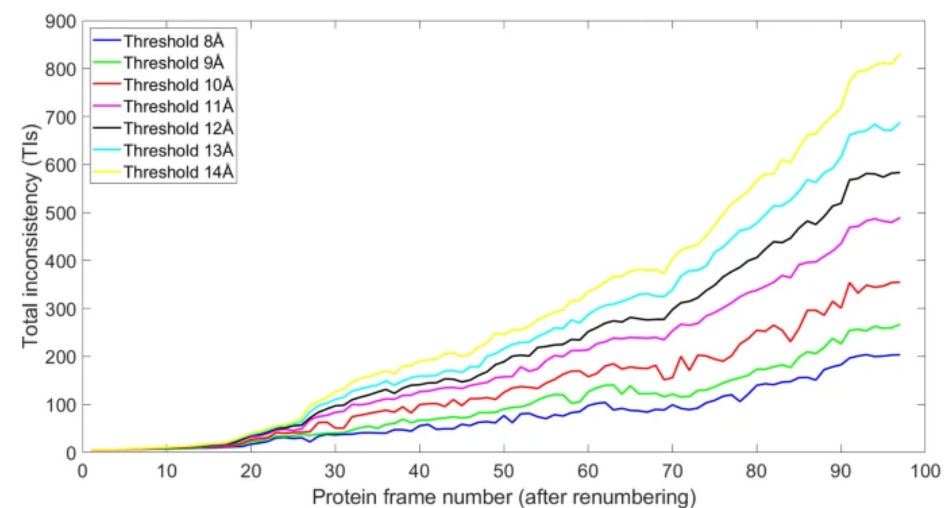
(TI) for Titin configurations during the SMD simulations
