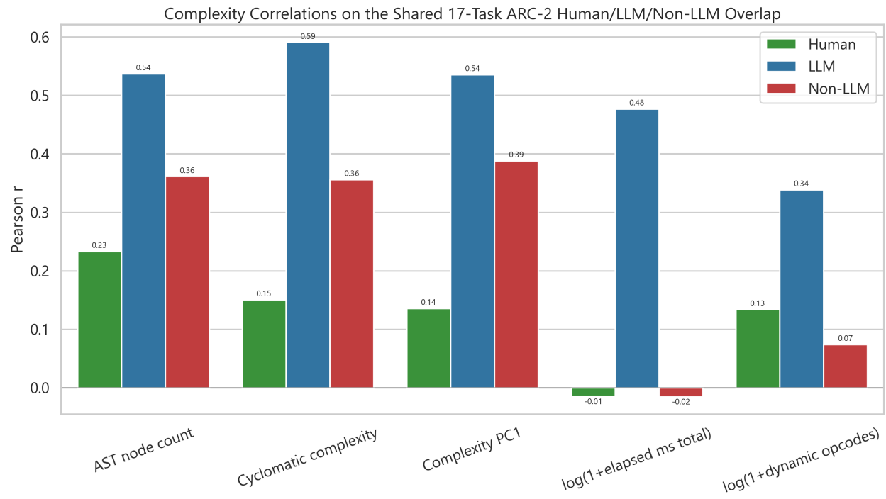
Figure 2: Human vs LLM vs non-LLM complexity comparisons on the shared 17-task ARC-2 overlap.
