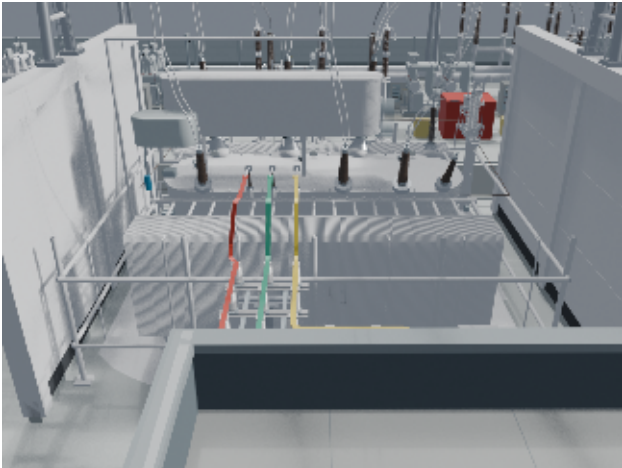
T1 rear / fans
