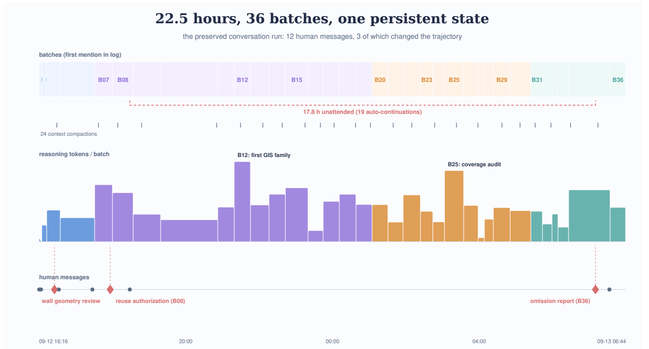
Figure 7. Session anatomy of the preserved 22.5-hour conversation run. Top: batch timeline (first mention in the log), the 17.8-hour unattended span, and the 24 context compactions. Middle: reasoning-output tokens per batch (a billing-reported proxy for reasoning effort), peaking at abstraction events rather than at the largest geometry. Bottom: the twelve substantive human messages; the three highlighted changed the trajectory.
