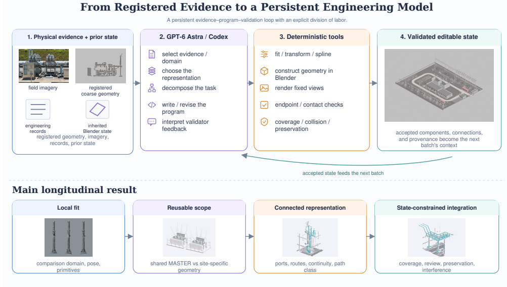
Figure 1. AstraBuild as a persistent evidence-program-validation workflow. Registered physical evidence and inherited engineering state condition a model-authored or model-revised operation; deterministic tools execute geometry construction and task-specific checks; accepted output becomes part of the next reconstruction context. The lower progression previews the paper’s longitudinal result: the common loop persists while additional representation and integration decisions appear as dependencies accumulate.
