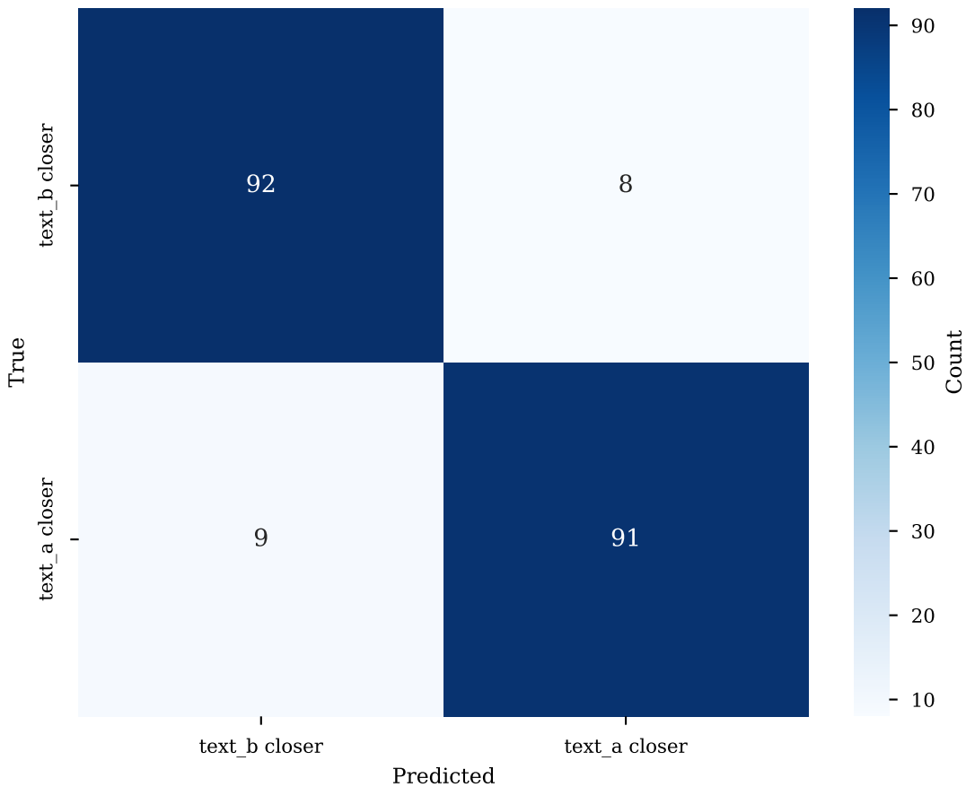
Confusion Matrix - Proposed Model
