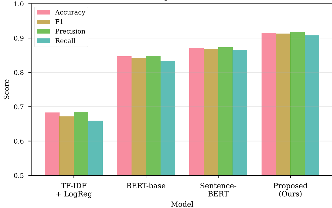
Model Comparison - All Metrics
