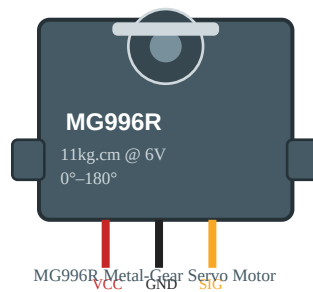
Fig. 1.3 – MG996R Metal-Gear Servo (×6)
