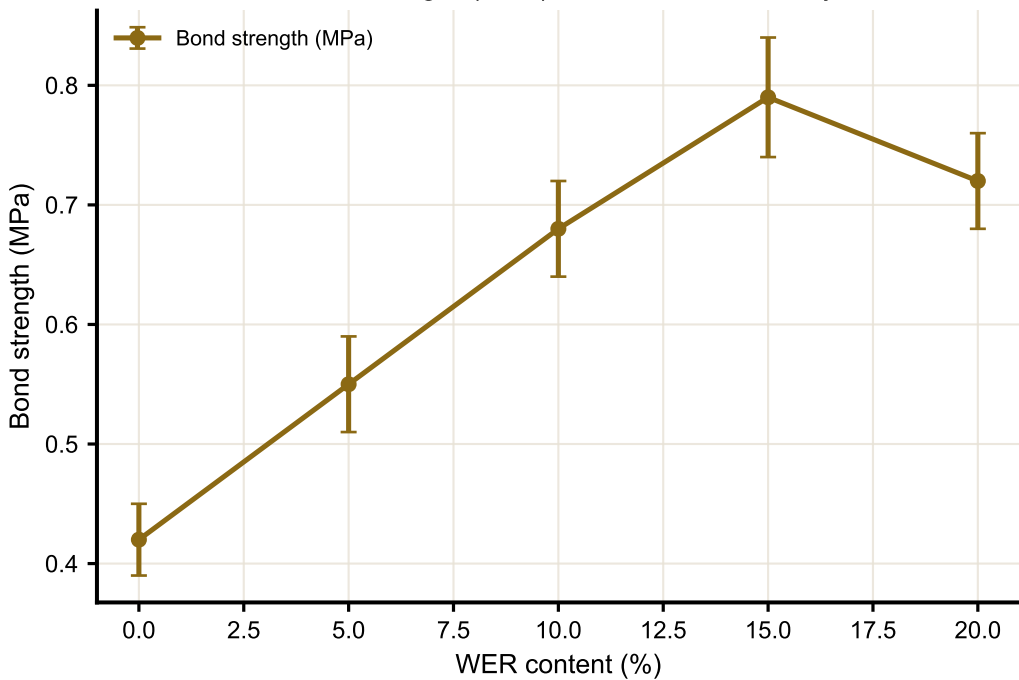
Bond strength (MPa) trend with uncertainty
