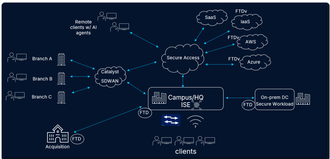
Use Case 4 — reference solution diagram (extend TrustSec to the acquired site via FTD inline SGT tagging; Duo Directory)
