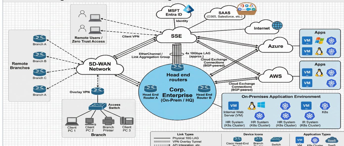
Architecture Design Clinic — Reference Network Diagram (current customer environment)
