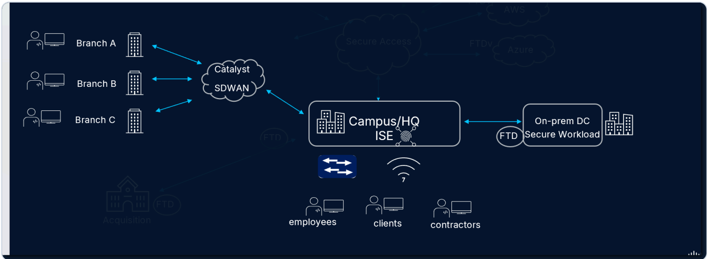
Use Case 1 — proposed final design (Segmentation: ISE + SGT across Campus/HQ, SD-WAN branches, on-prem DC Secure Workload)
