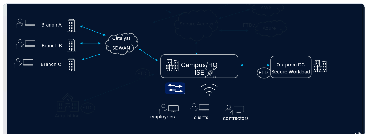
Use Case 1 — reference solution diagram (Segmentation: ISE + SGT across Campus/HQ, SD-WAN branches, on-prem DC Secure Workload)
