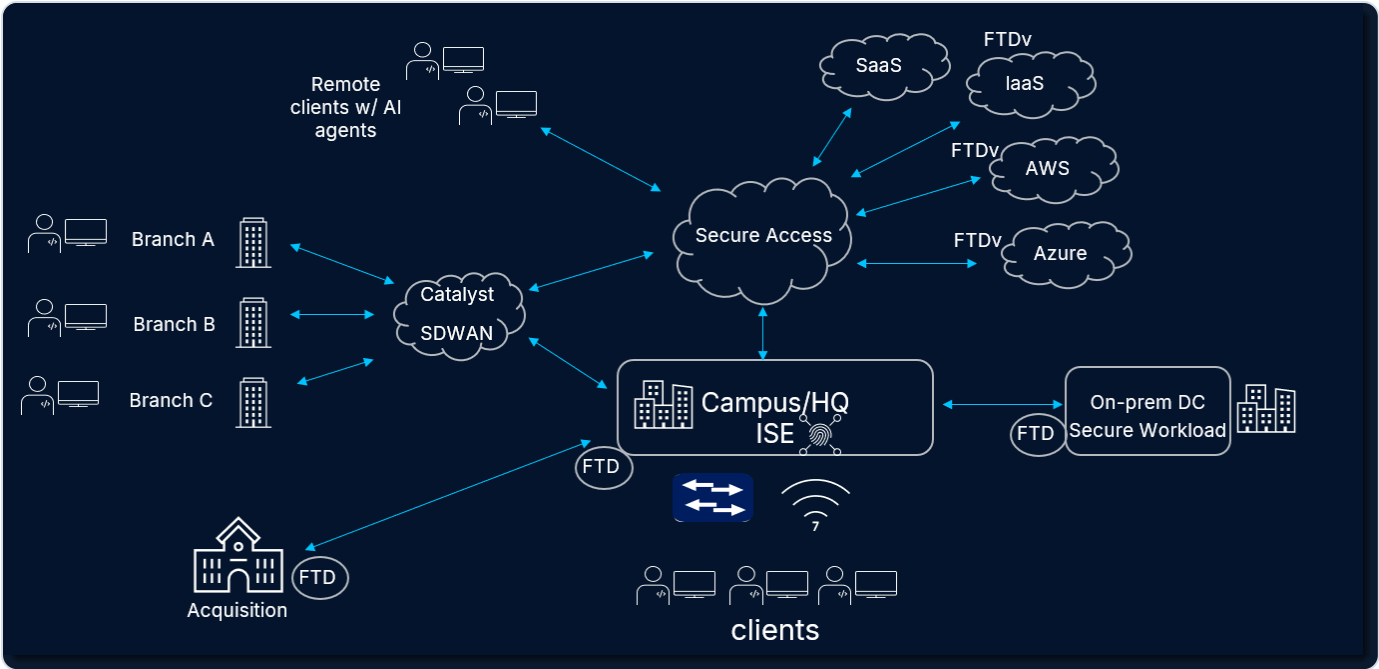
Use Case 4 — reference solution diagram (extend TrustSec to the acquired site via FTD inline SGT tagging; Duo Directory)
