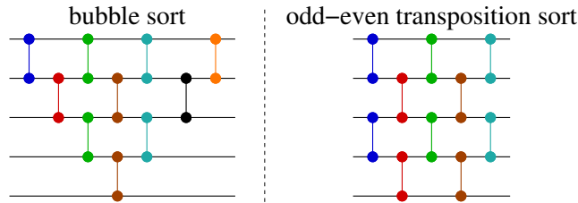
Figure 2: Sorting networks for a linear array
