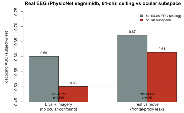
Figure 9: Real EEG ( eegmldb ). Full-EEG ceiling (grey) versus ocular-subspace (red) decoding AUC. Left-versus-right imagery is at chance in the ocular subspace; rest-versus-move leaks through the channel proxy.
