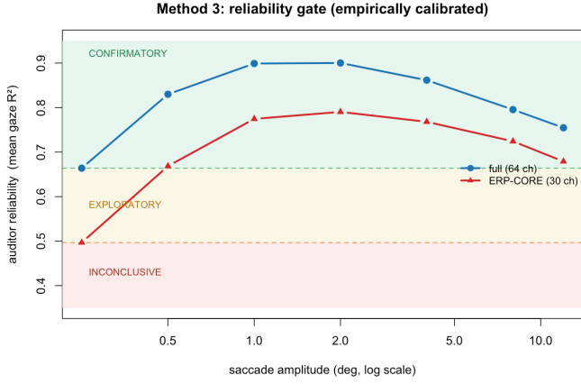
Fig. 7. Reliability gate. The sparse 30-channel ERP-CORE subset drops into the exploratory zone at the fixational extreme, while the full 64-channel montage stays confirmatory throughout.
