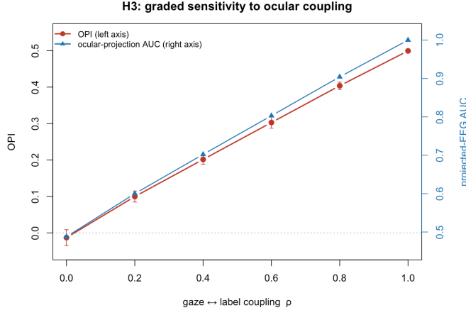
Fig. 5. Graded sensitivity: OPI (red, left axis) and ocular-projection AUC (blue, right axis) rise monotonically with the gaze-label coupling.
