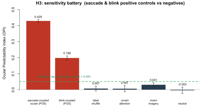
Fig. 4. H3 sensitivity battery. The two positive controls (red: saccade- and blink-coupled ocular) exceed every negative control; all negative controls sit at or below the calibrated neural-leakage margin (green dashed). Error bars are \pm SD over 12 studies.
