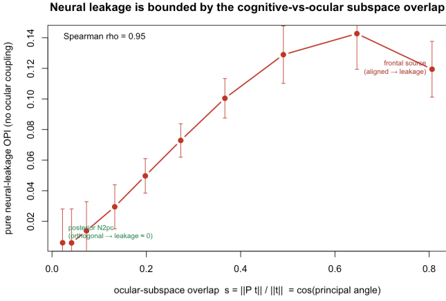
Fig. 8. Neural leakage versus the cognitive-vs-ocular subspace overlap s = \cos \theta . Pure neural-leakage OPI rises monotonically with s ( \rho = 0.95 ) and is \approx 0 for a posterior (orthogonal) source.
