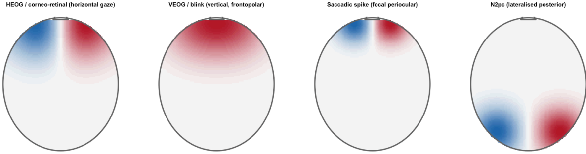
Fig. 3. Physically grounded source topographies in the forward model: the antisymmetric horizontal corneo-retinal (HEOG) field, the symmetric frontopolar vertical/blink field, the focal periocular saccadic spike, and the lateralized posterior N2pc. Red/blue denote opposite polarity.
