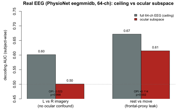
Figure 9: Real EEG (eegmldb). Full-EEG ceiling (grey) versus ocular-subspace (red) decoding AUC. Left-versus-right imagery is at chance in the ocular subspace; rest-versus-move leaks through the channel proxy.
