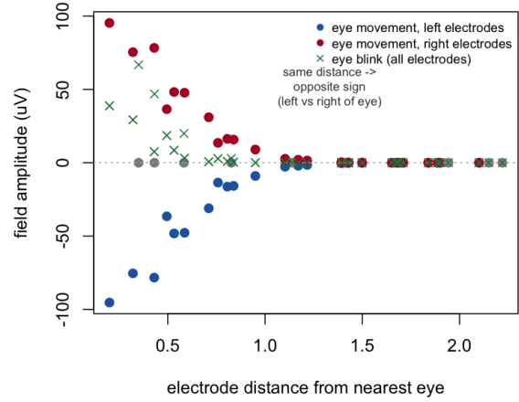
Field vs distance and position
