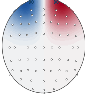
Electric field of a 10-deg eye movement (uV)
