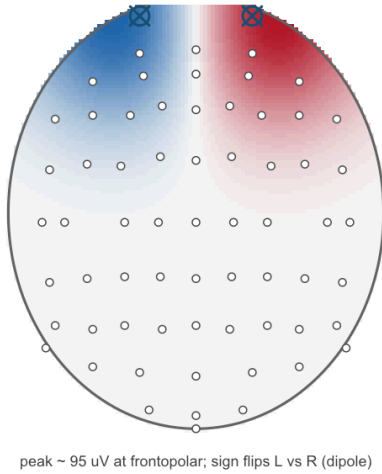
Fig. 1. The electric field of an eye movement depends on electrode position. Left: scalp field of a 10° horizontal eye movement over the 64-channel montage (peak \approx 95 \mu\text{V} at frontopolar sites; sign reverses left/right of the eyes—a dipole). Right: field amplitude versus each electrode’s distance from the nearest eye. At a given distance the sign depends on which side of the eyes the electrode sits (blue vs. red); an eye blink (green) imposes a distinct, symmetric, one-signed field that also decays with distance. This position- and artifact-dependence is why the auditor is montage-matched.
