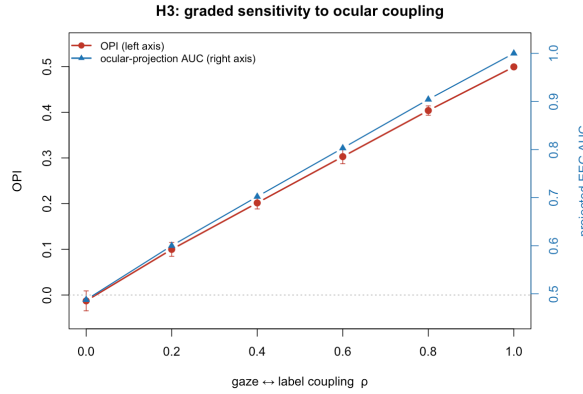
Figure 5: Graded sensitivity: OPI (red, left axis) and ocular-projection AUC (blue, right axis) rise monotonically with the gaze-label coupling.
