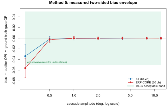
Figure 6: Measured two-sided bias envelope: auditor OPI minus ground-truth-gaze OPI versus saccade amplitude. Deviations are negative (conservative) and confined to the fixational extreme on the sparse montage.
