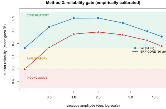
Figure 7: Reliability gate. The sparse 30-channel ERP-CORE subset drops into the exploratory zone at the fixational extreme, while the full 64-channel montage stays confirmatory throughout.
