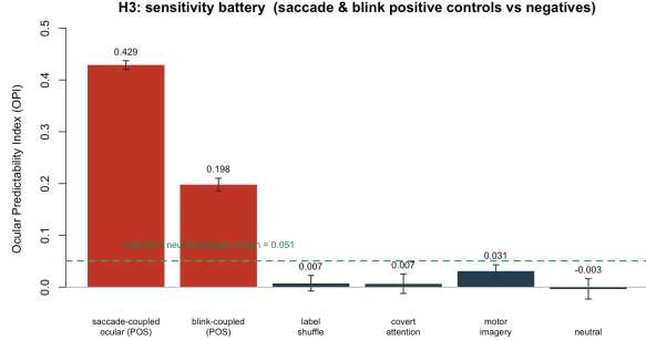
Figure 4: H3 sensitivity battery. The two positive controls (red: saccade- and blink-coupled ocular) exceed every negative control; all negative controls sit at or below the calibrated neural-leakage margin (green dashed). Error bars are \pm SD over 12 studies.
