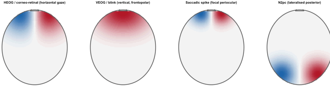
Figure 3: Physically grounded source topographies in the forward model: the antisymmetric horizontal corneo-retinal (HEOG) field, the symmetric frontopolar vertical/blink field, the focal periocular saccadic spike, and the lateralized posterior N2pc. Red/blue denote opposite polarity.
