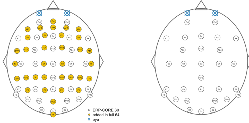
Figure 2: Montages. The full auditor montage (left, 64 channels) contains the 30-channel ERP-CORE set (white) plus 34 further 10–10 electrodes (yellow), including denser near-eye frontal coverage that the 30-channel target montage (right) lacks; this density gap drives the reliability gate. Eyes marked in blue.
