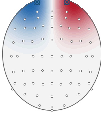
Electric field of a 10-deg eye movement (uV)
