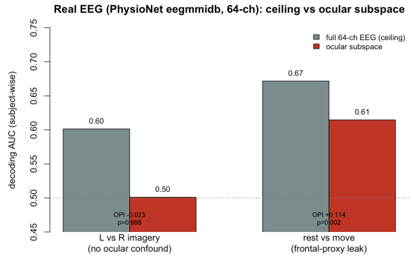
Figure 9: Real EEG (eegmddb). Full-EEG ceiling (grey) versus ocular-subspace (red) decoding AUC. Left-versus-right imagery is at chance in the ocular subspace; rest-versus-move leaks through the channel proxy.
