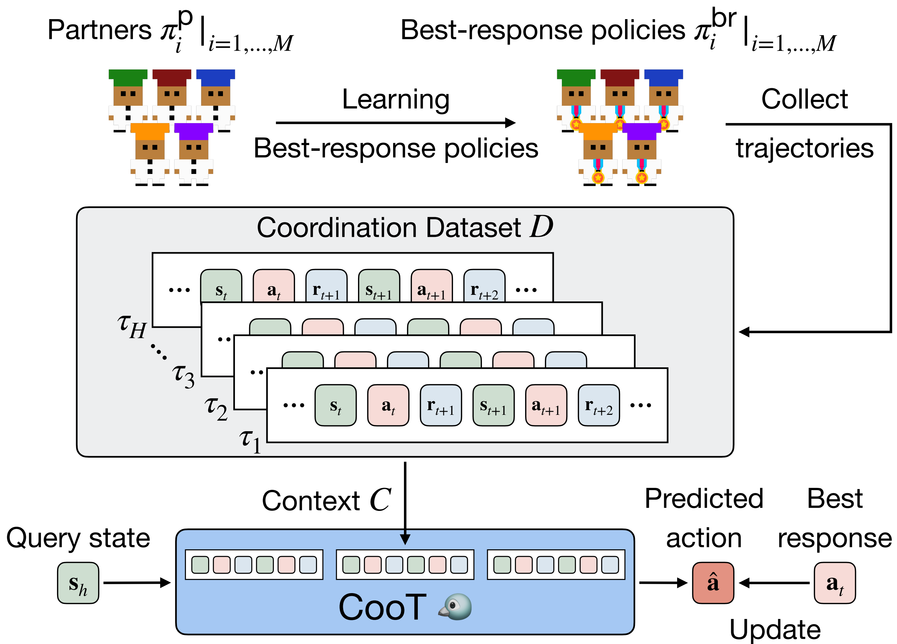
(a) Constructing and learning from coordination dataset
