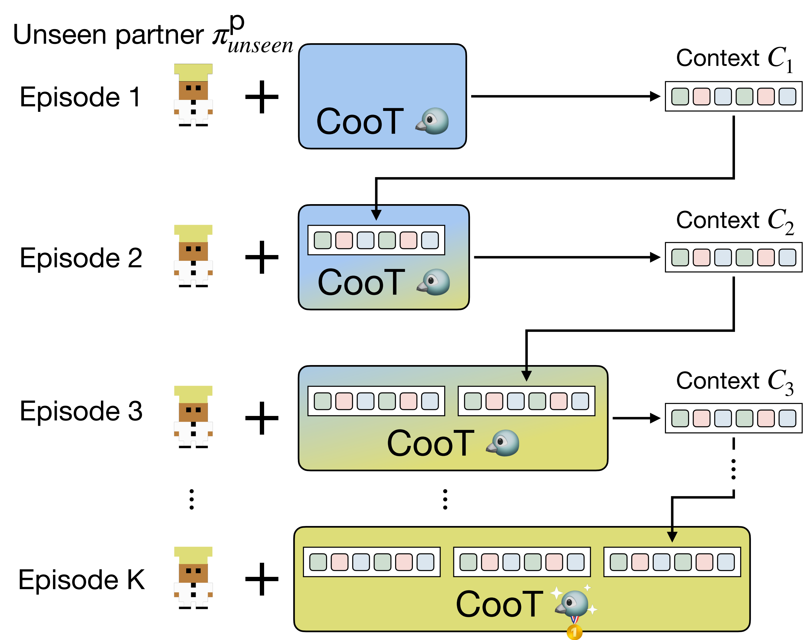
(b) In-context coordination
