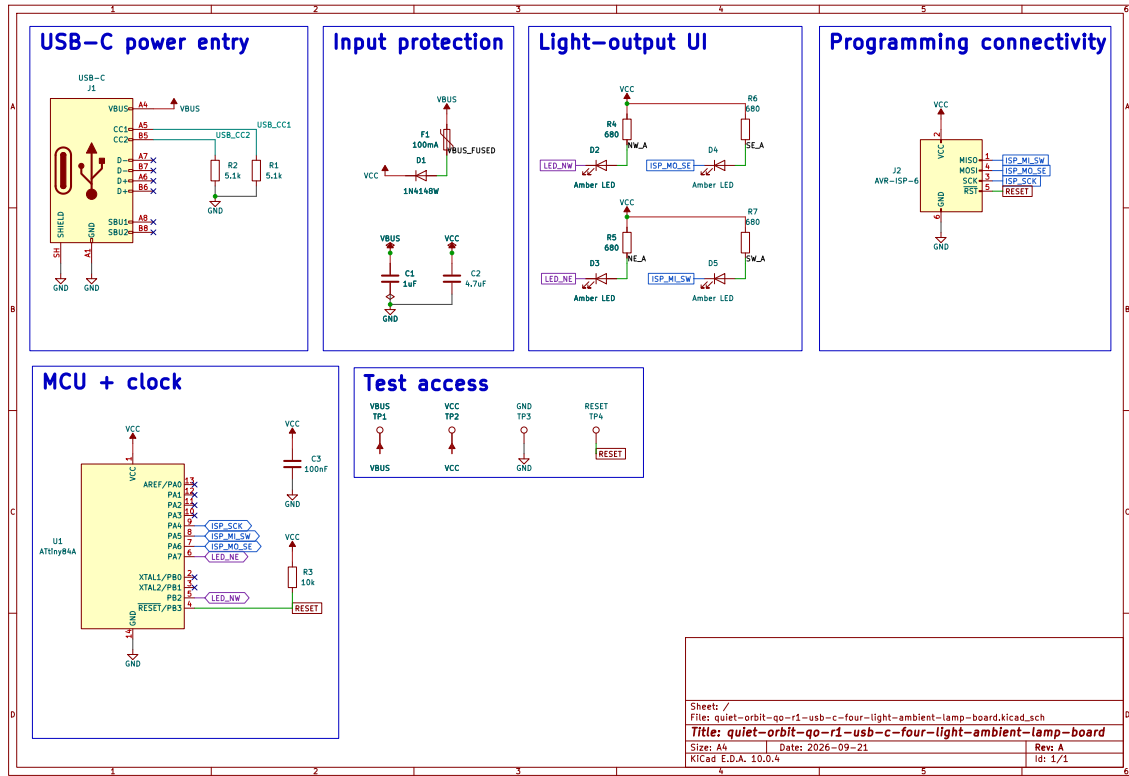
Figure 2: Full schematic sheet, scaled to page width. Full size in docs/schematic.pdf.
