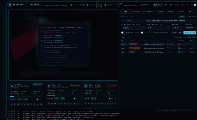
IMPORT CEREMONY: SCAN, TWO APPROVALS, PINNED KEY, SIGNATURE, DIGEST, LOAD
