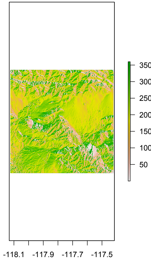
aspect
