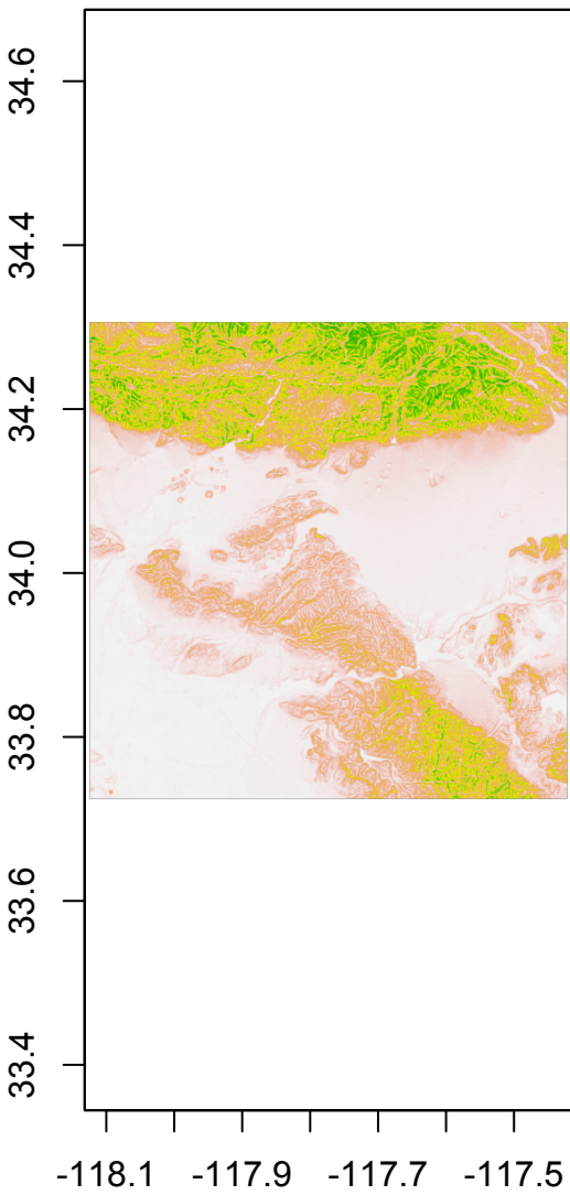
slope
