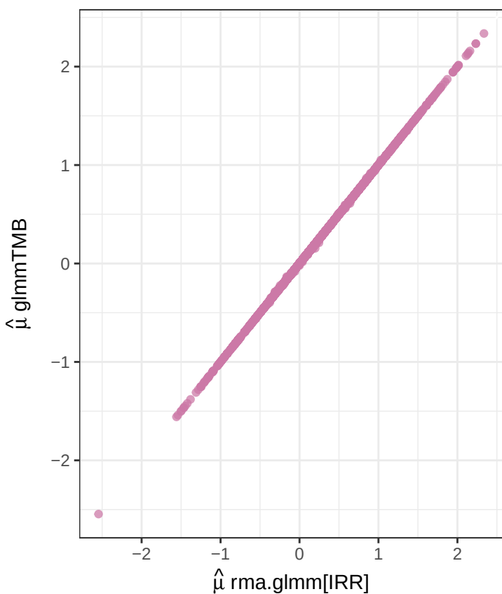
Poisson–Normal models agreement
