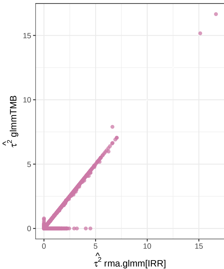
Poisson–Normal models agreement
