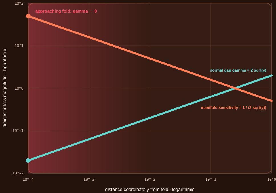
FIGURE 31 — Analytical illustration of the dimensionless fold normal form: normal attraction tends to zero and slow-branch sensitivity diverges as the dimensionless distance coordinate y approaches the fold; this is exact geometry for the displayed normal form, not a measured or universal online threshold.
