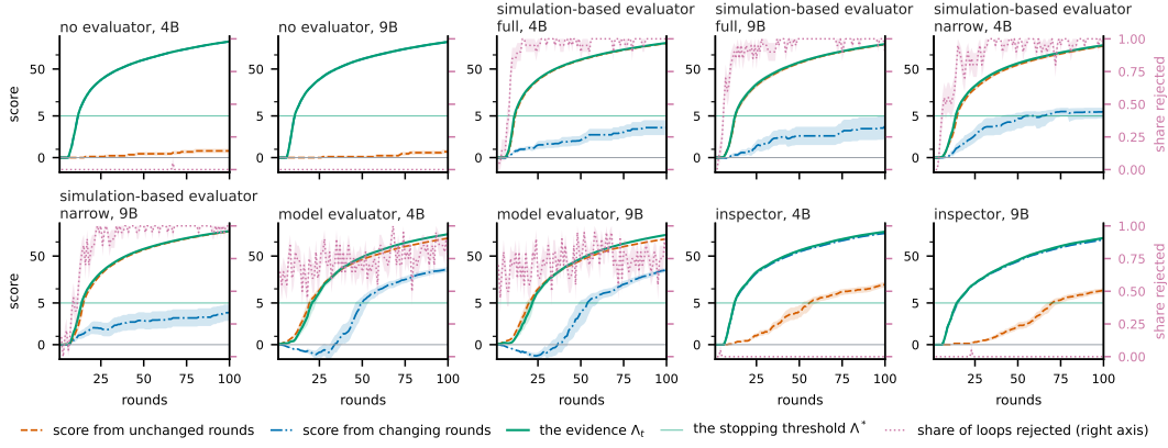
Figure I.10: The sources of the evidence on every cruise-control scenario, namely the score accumulated by unchanged rounds, the score accumulated by changing rounds, and the evidence \Lambda_t against the threshold \Lambda^* , each a mean over the loops with a band of one standard error, with the share of loops rejected at each round on the right axis.
