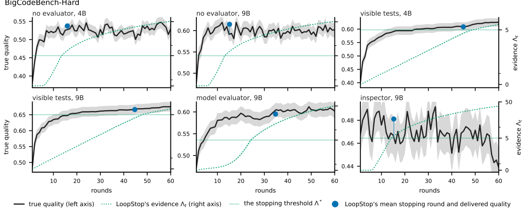
Figure I.8: Every scenario of BigCodeBench-Hard by round, drawn as in Figure 2, with the true quality on the left axis and LOOPSTOP’s evidence \Lambda_t on the right, each a mean over the loops with a band of one standard error, the threshold \Lambda^* , and LOOPSTOP’s mean stopping round and delivered quality.
