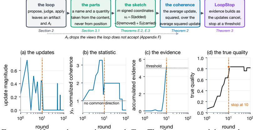
Figure I.1: From an artifact to the stopping round. Top . The five stages and the result governing each stage. Bottom . A single cruise-control loop, with the update magnitudes, y_k , the sum \Lambda_t against its threshold, and the true quality, with the round on a logarithmic axis.
