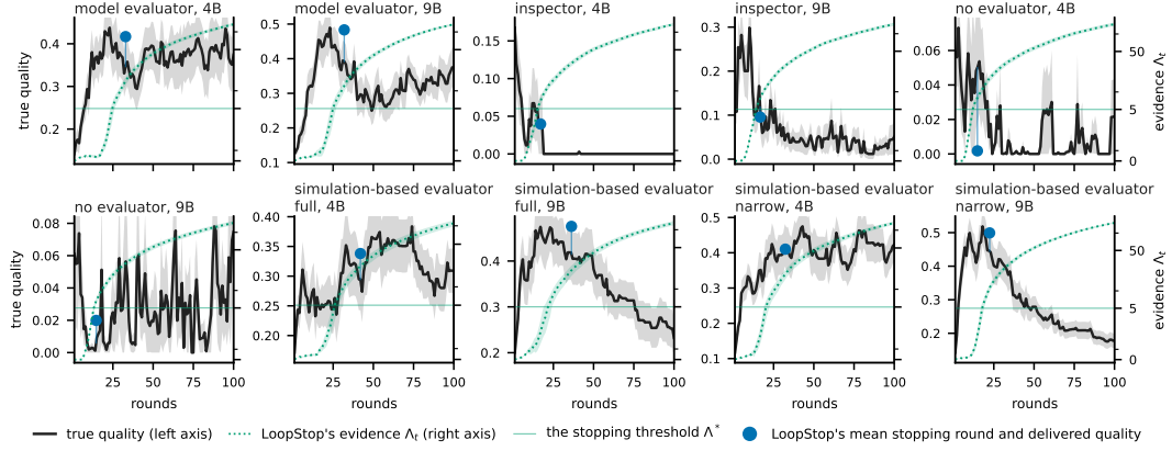
Figure I.6: Every cart-pole scenario by round, drawn as in Figure 2, with the true quality on the left axis and LOOPSTOP's evidence \Lambda_t on the right, each a mean over the loops with a band of one standard error, the threshold \Lambda^* , and LOOPSTOP's mean stopping round and delivered quality.
