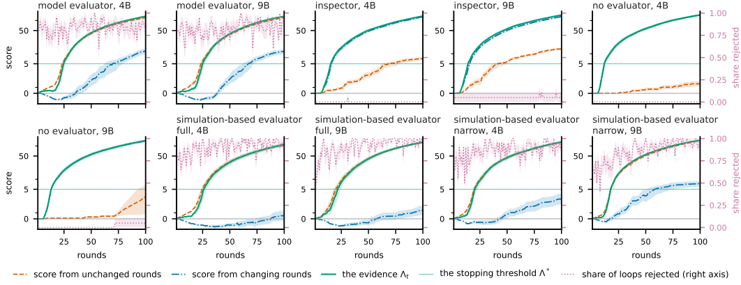
Figure I.11: The sources of the evidence on every cart-pole scenario, namely the score accumulated by unchanged rounds, the score accumulated by changing rounds, and the evidence \Lambda_t against the threshold \Lambda^* , each a mean over the loops with a band of one standard error, with the share of loops rejected at each round on the right axis.
