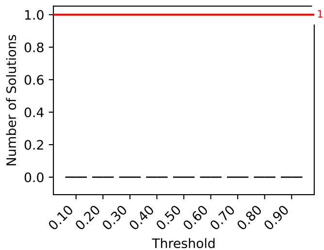
KnightTour-06-ext03
