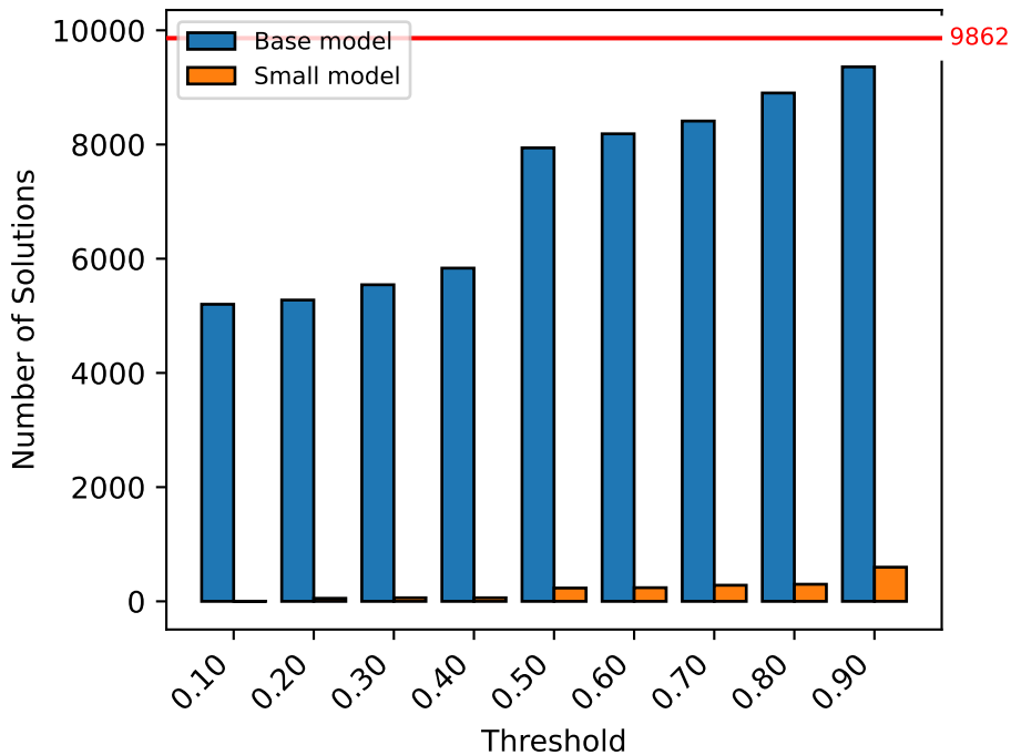
KnightTour-06-ext03
