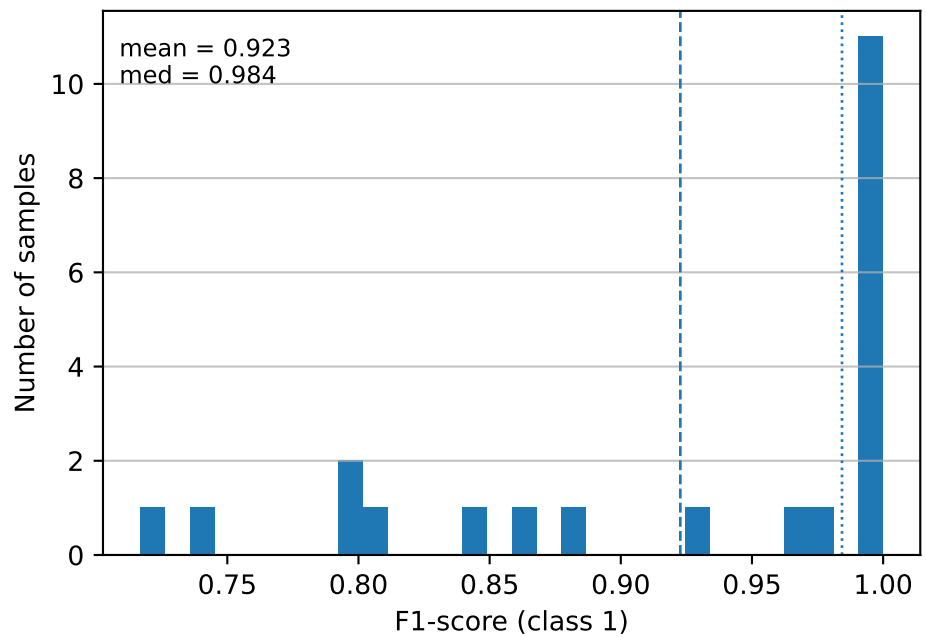
F1-score (class 1)
