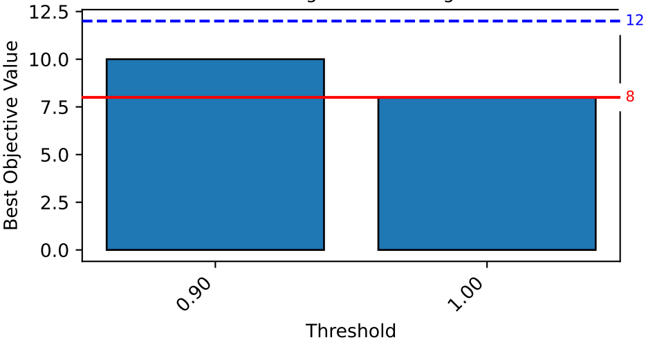
MultiAgentPathFinding
