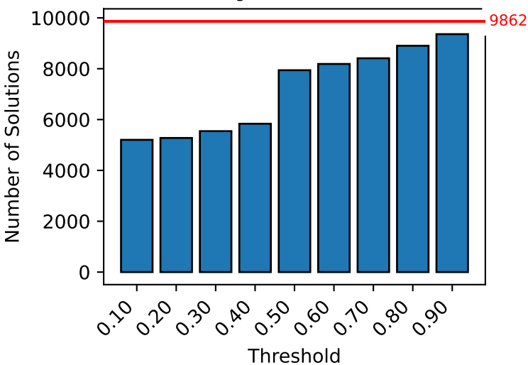
KnightTour-06-ext03
