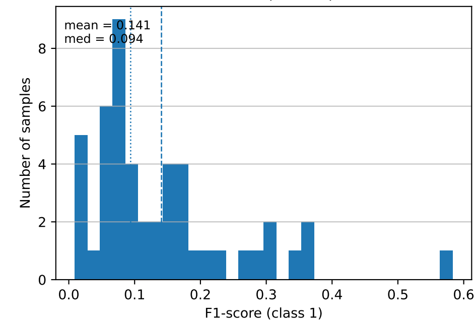
F1-score (class 1)
