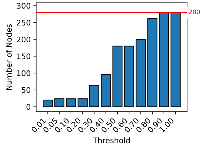
MultiAgentPathFinding
