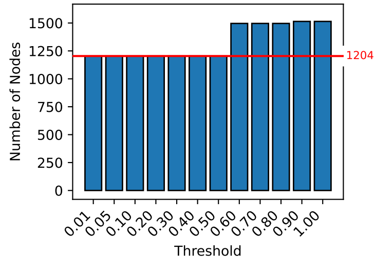
MultiAgentPathFinding
