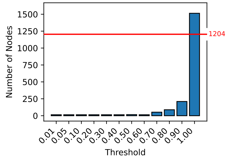
MultiAgentPathFinding
