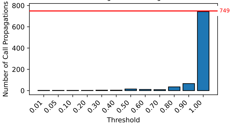
MultiAgentPathFinding
