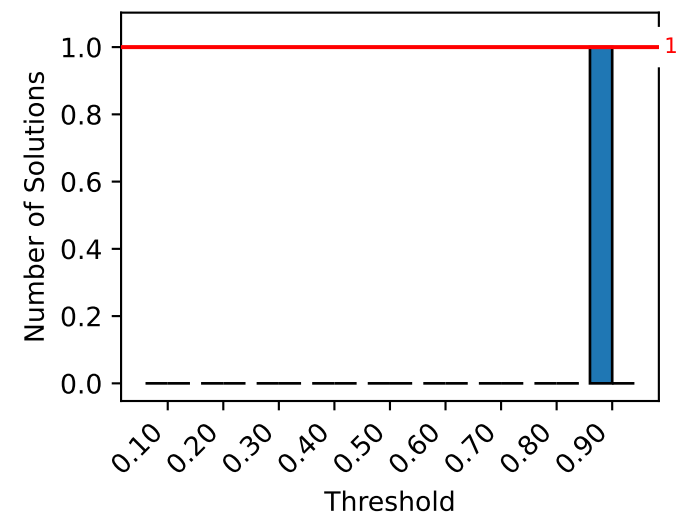
Queens-0009-m1
