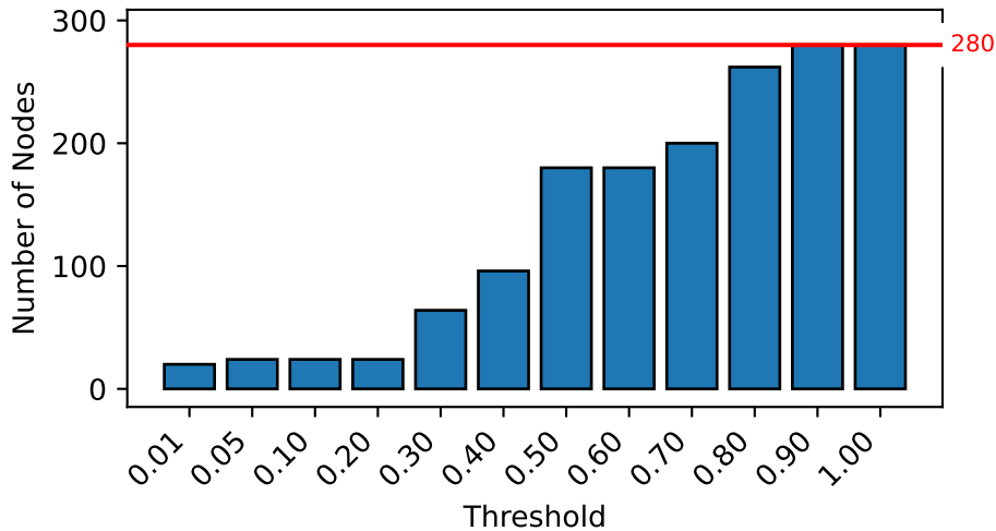
MultiAgentPathFinding
