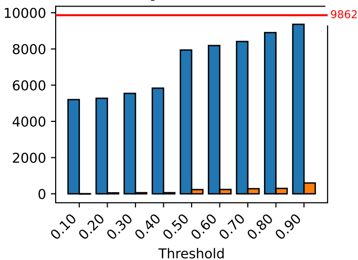
KnightTour-06-ext03
