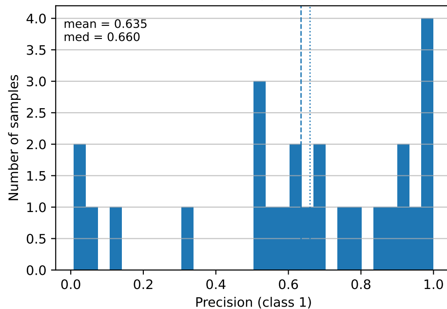
Precision (class 1)
