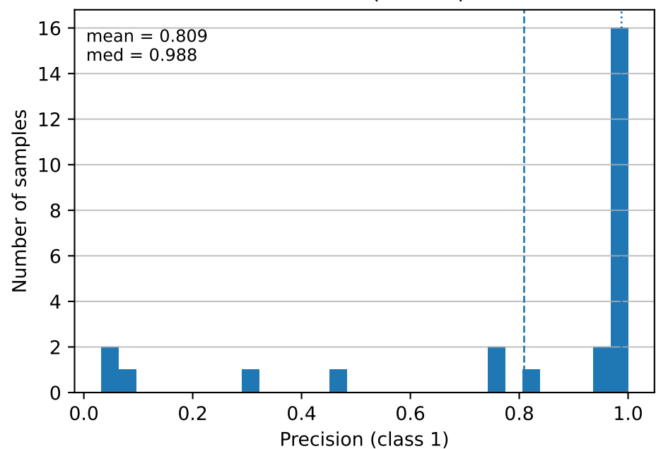
Precision (class 1)
