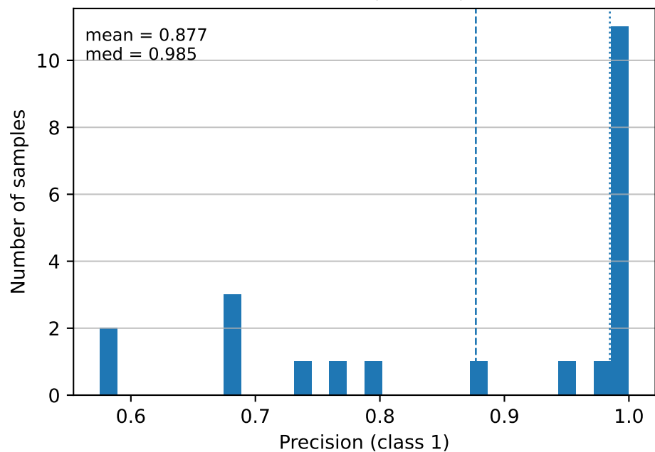
Precision (class 1)
