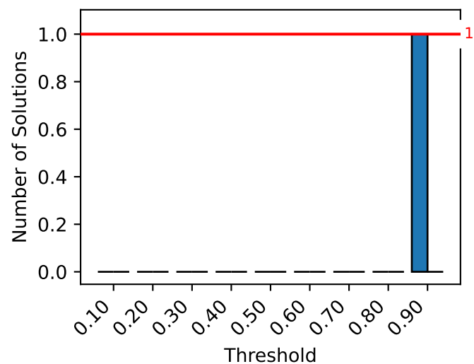
Kakuro-medium-062-sumdiff
