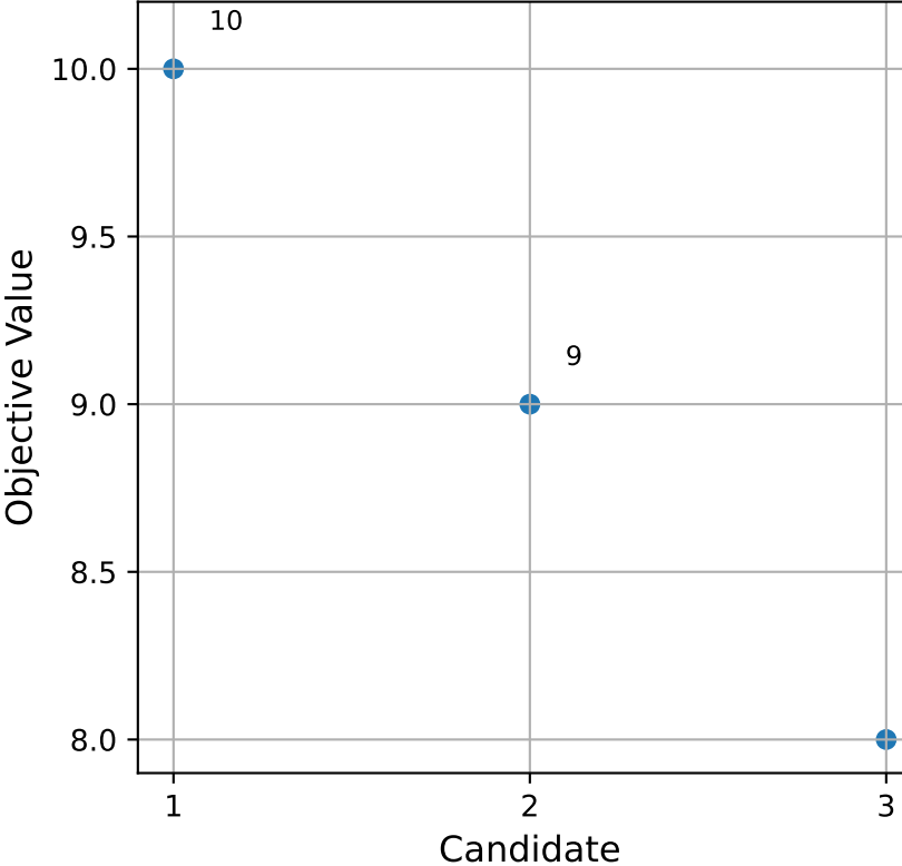
MultiAgentPathFinding
