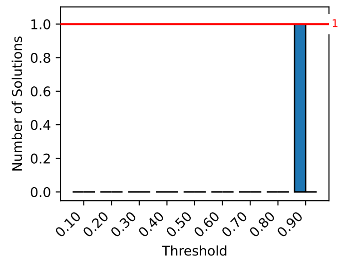
Kakuro-medium-086-sumdiff
