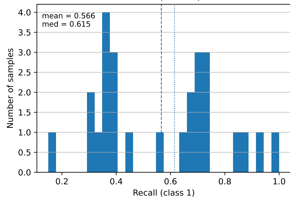
Recall (class 1)
