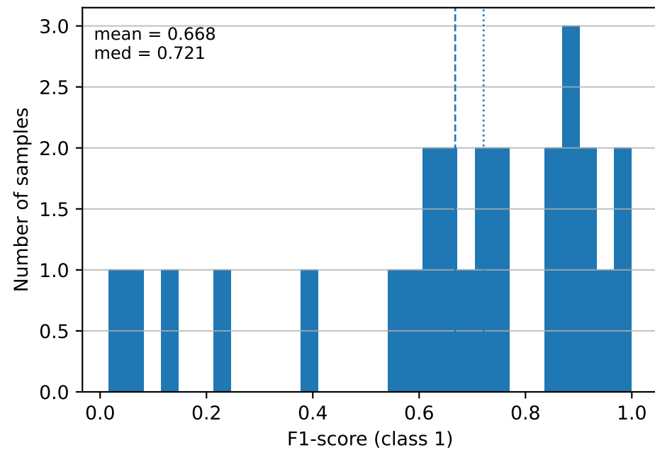
F1-score (class 1)
