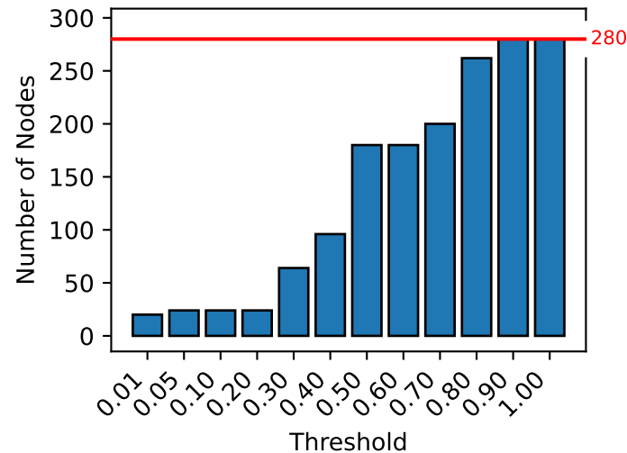
MultiAgentPathFinding
