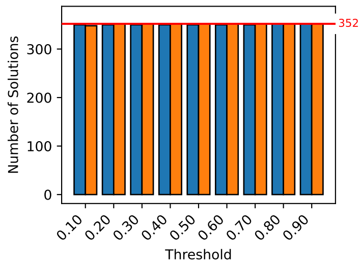
Queens-0009-m1
