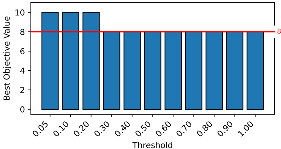
MultiAgentPathFinding
