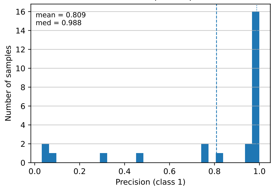
Precision (class 1)
