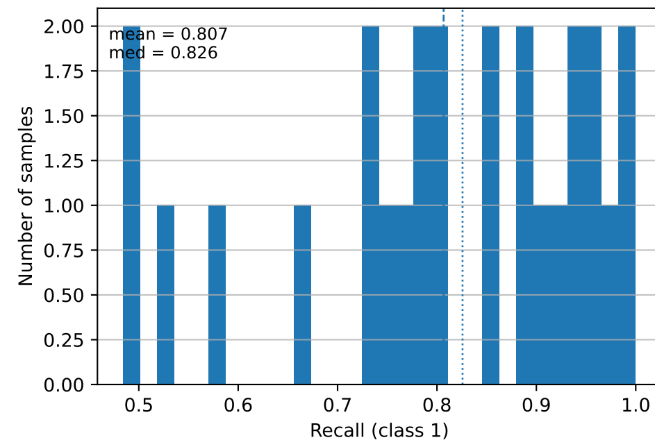
Recall (class 1)
