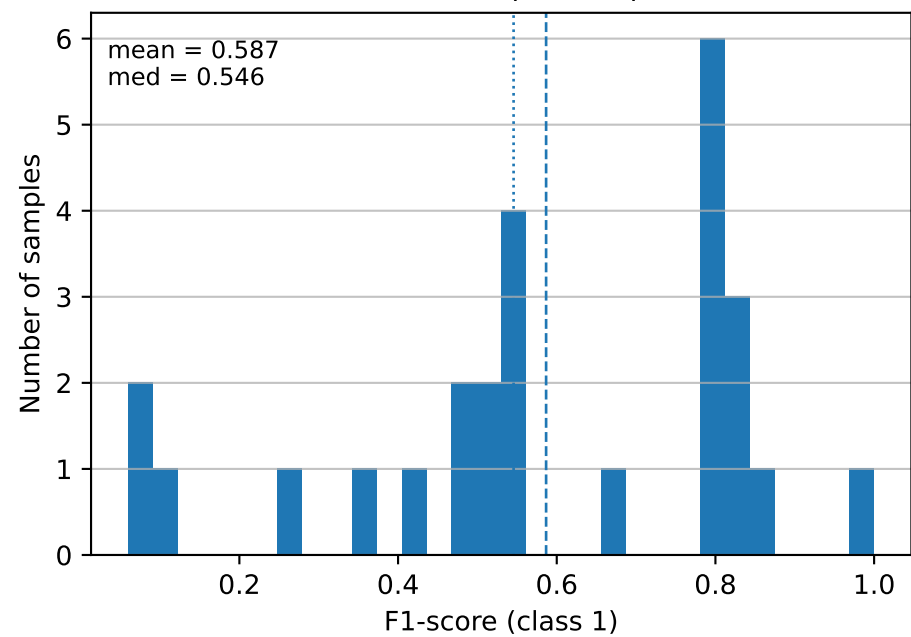
F1-score (class 1)
