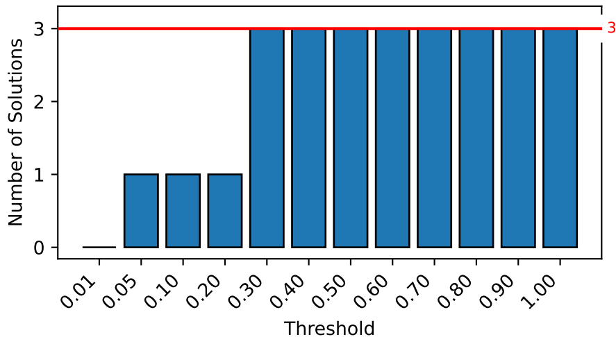
MultiAgentPathFinding
