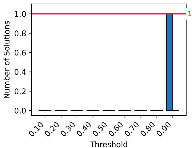
Kakuro-medium-035-sumdiff
