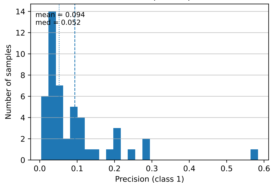
Precision (class 1)
