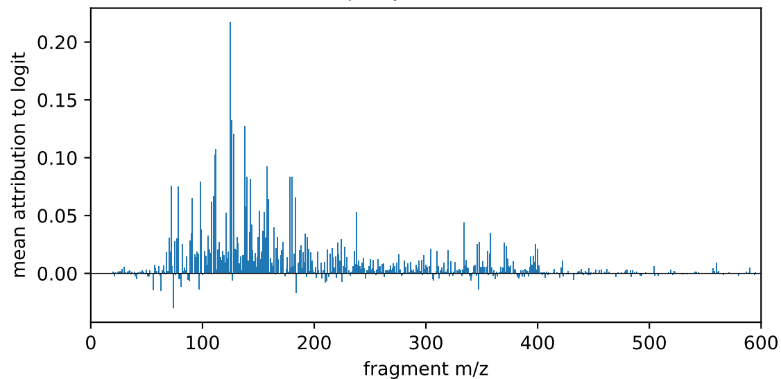
bit 1750: c(c)c frequency 0.81, AUC 0.87
