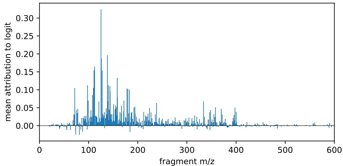
bit 1476: O=S frequency 0.17, AUC 0.89
