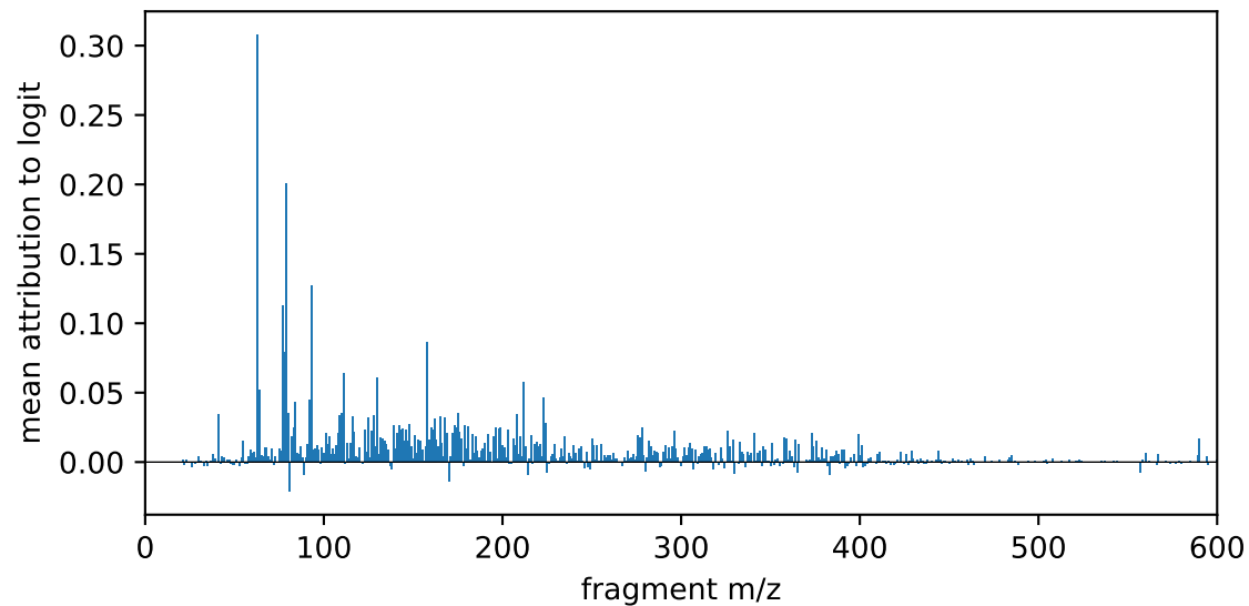
bit 1683: Cl frequency 0.12, AUC 0.89
