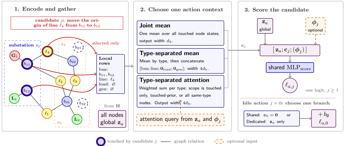
Figure 4.12: Candidate-action scoring for an endpoint-move candidate. The encoder provides the global graph embedding \mathbf{z}_a and physical node states \mathbf{H} . Violet outlines mark the only rows gathered for the local context: both busbars of the modified substation and the touched explicit-line node. One pooling construction then produces \mathbf{c}_j . The static descriptor \phi_j may be appended before the shared non-idle scorer. The idle action uses either zero local context in that scorer or a dedicated scorer.
