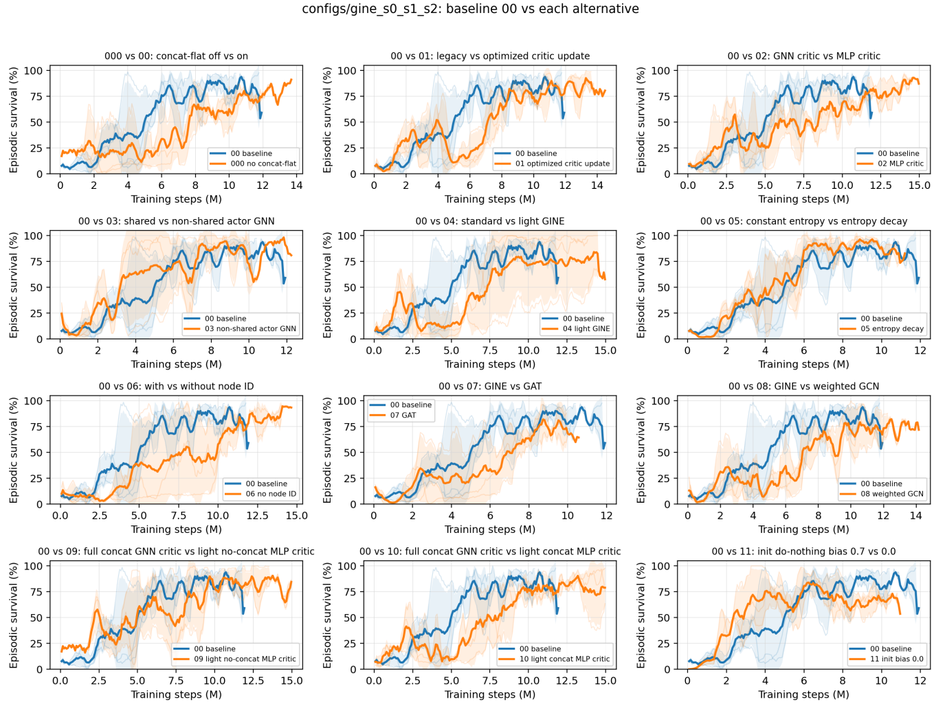
Figure 2.5: Heavy-GINE best-search 2 survival comparisons. Each subplot compares the best_00 heavy concat-flat GINE baseline against one controlled alternative from configs/gine_s0_s1_s2 .
