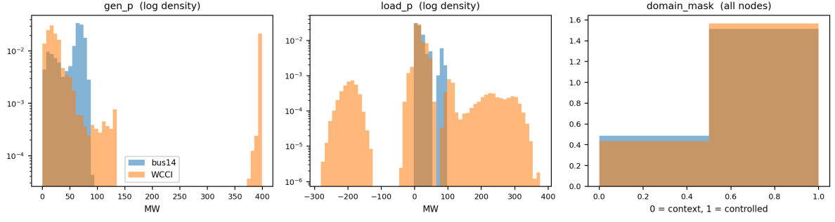
Figure A.9: Tail behaviour of the power channels on log density, and the structural domain_mask . WCCI carries a generator pinned near its 399 MW rating and a load region reaching -281 MW, neither of which occurs anywhere on bus14 : a frozen encoder has no calibration for either. domain_mask is near-identical on the two grids, so the small difference in Table 7.1 carries no signal.
