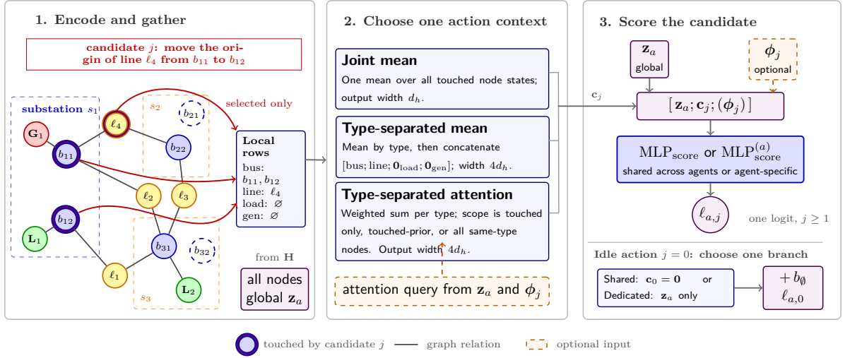
Figure 5.9: Candidate-action scoring for an endpoint-move candidate. The encoder provides the global graph embedding \mathbf{z}_a and physical node states \mathbf{H} . Violet outlines mark the only rows gathered for the local context: both busbars of the modified substation and the touched explicit-line node. One pooling construction then produces \mathbf{c}_j . The static descriptor \phi_j may be appended before the shared non-idle scorer. The idle action uses either zero local context in that scorer or a dedicated scorer.
