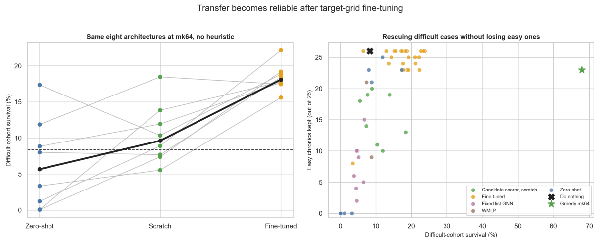
Figure 9.4: Effect of target-grid training. Grey lines join the same architecture in the left panel. The black cross and green star in the right panel are do nothing and the greedy k = 64 reference.
