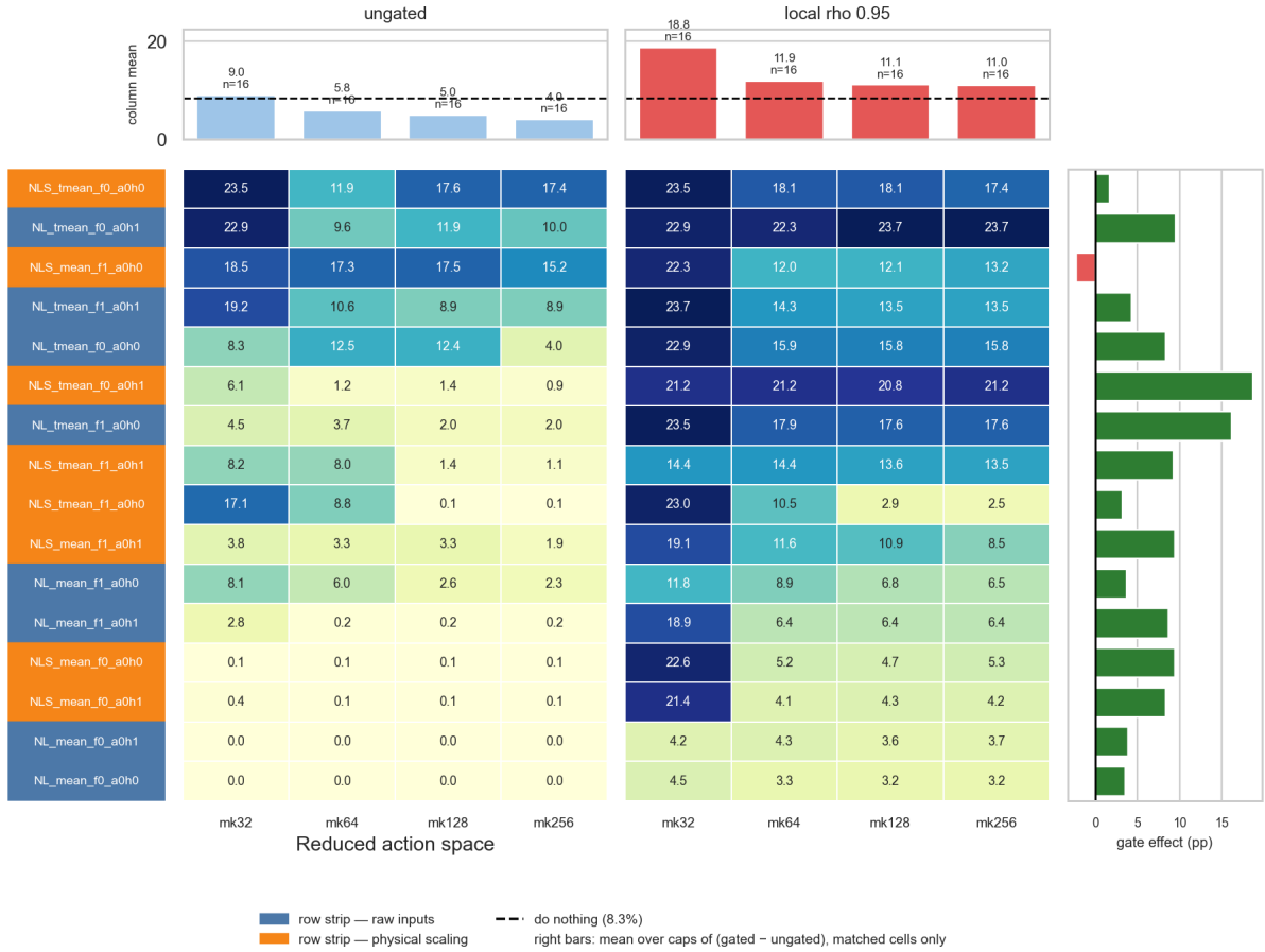
Figure A.12: Zero-shot difficult-cohort survival across input, pooling, descriptor, idle-head and action-space choices.
