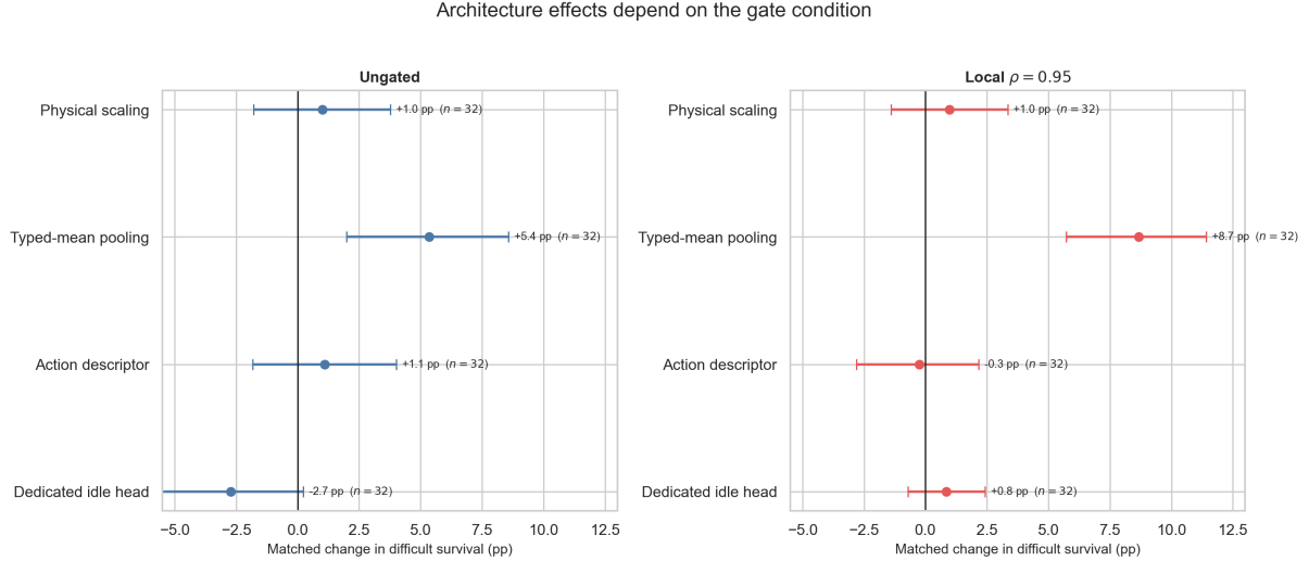
Figure 9.2: Matched architecture effects on the difficult cohort, shown separately for ungated actors and the local- \rho = 0.95 heuristic. Positive values improve survival. Error bars are bootstrap intervals over matched architecture cells; n is the number of available pairs.
