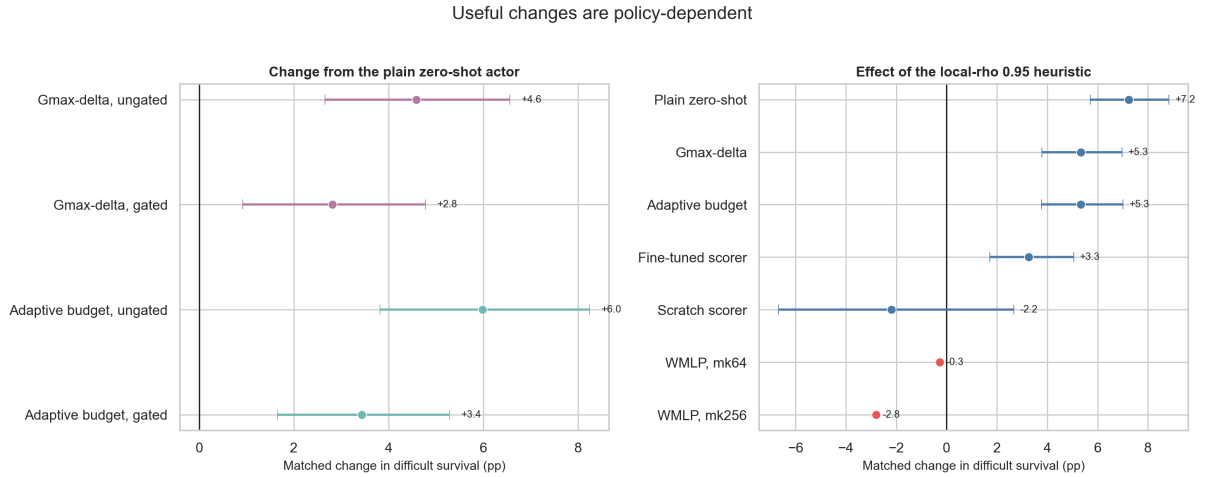
Figure 9.3: Matched changes on the difficult cohort. Positive values are better. The Gmax-delta and adaptive-budget blocks are compared with the same plain zero-shot architectures.
