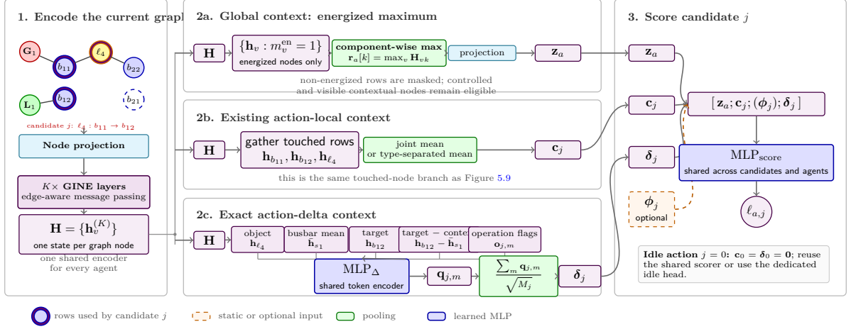
Figure 5.10: Gmax-delta extension of Figure 5.9. The shared GINE encoder returns node states \mathbf{H} . The upper branch builds the global vector by maximum pooling over energized nodes; the middle branch keeps the original touched-node context \mathbf{c}_j ; and the lower branch encodes each exact object modification and aggregates the resulting tokens into \delta_j . The shared scorer receives all three state-dependent contexts and, optionally, the static descriptor \phi_j . No post-action graph or power flow is computed.
