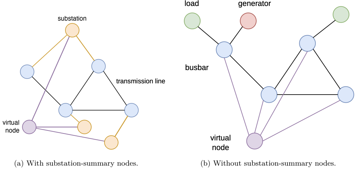
Figure 3.7: Virtual-node graph readout, shown for both definitions of the summary set \mathcal{V}_{\text{sum}} in Equation 3.23. The purple node aggregates that set and its final embedding replaces terminal node pooling. Every purple edge is directed toward the virtual node, which sends no message back. In (a) the substation-summary augmentation of Section 3.3.2 is enabled, so the virtual node attaches to the orange substation nodes and reaches the busbars only through them, which gives a two-level hierarchy busbar \rightarrow substation \rightarrow virtual node. In (b) the augmentation is disabled and the virtual node attaches directly to every included busbar. In neither case does it connect to generator, load, or transmission-line nodes.
