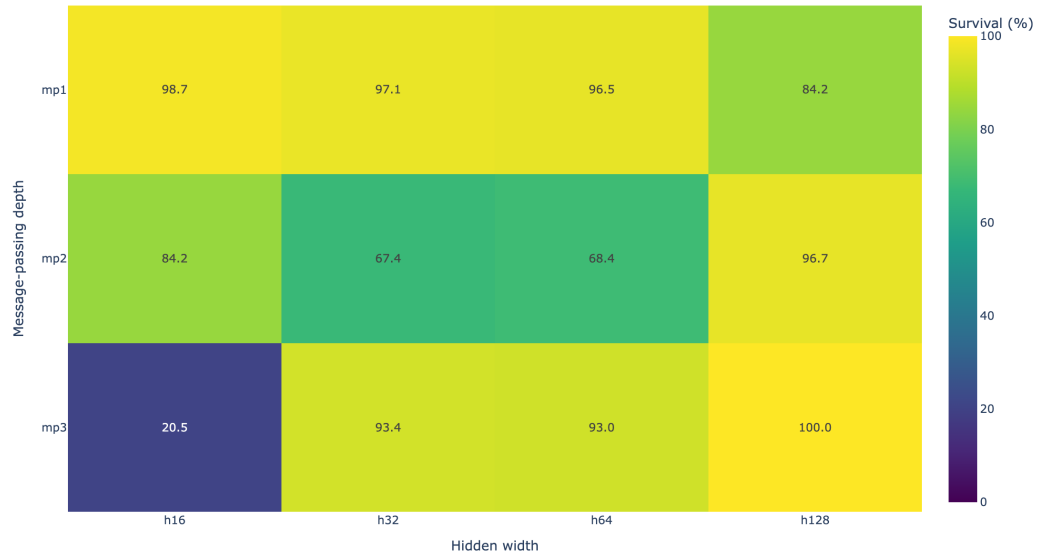
Figure 4.2: Screen A. The same twelve cells as a heatmap of the full-test survival of each run’s best checkpoint.
