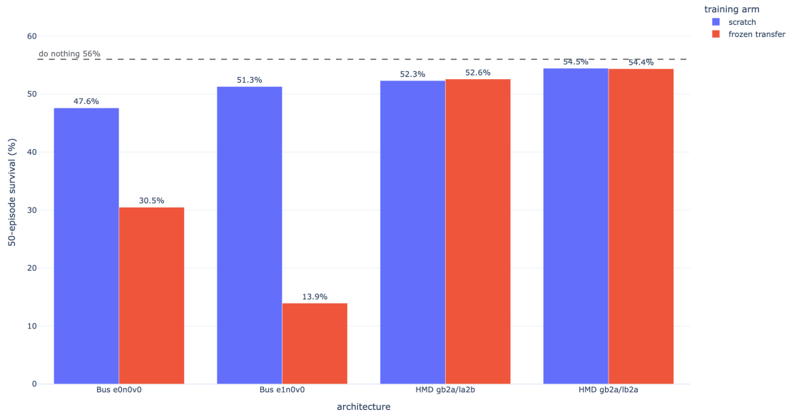
Figure 6.7: 50-episode full-test survival of the best checkpoint, by architecture and training arm, with uncorrected inputs and one seed. The dashed line is the do-nothing policy at 56%.
