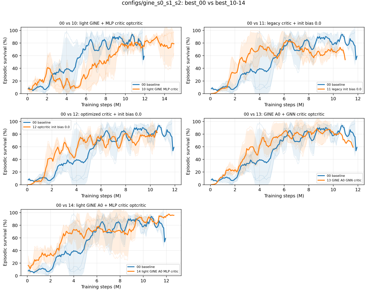
Figure 2.4: Seed-aggregated test episodic survival for GINE best_00 against best_10–best_14 .
