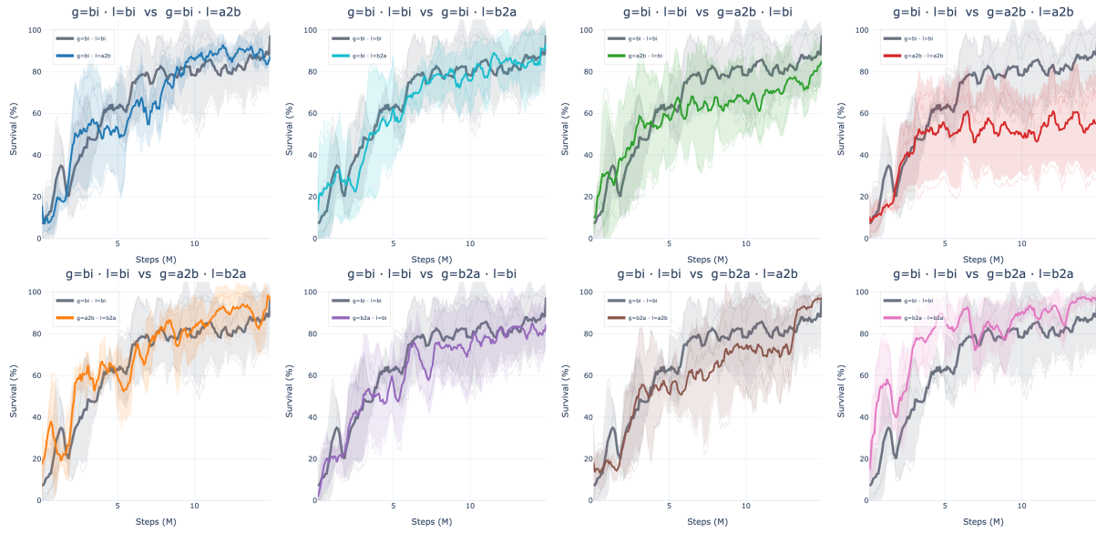
Figure 4.9: Screen D. Test episodic survival during training, one panel per direction pair against the bidirectional baseline in grey. Thin lines are the three seeds, the thick line is their mean, and the band is one standard deviation.
