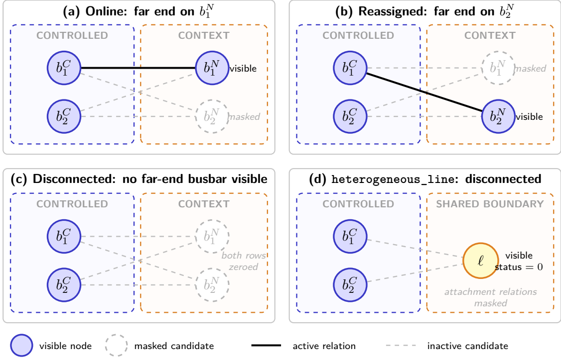
Figure 5.4: Dynamic visibility with a fixed candidate graph. In the direct-edge schemas, reassignment changes the active pair and visible far-end busbar; disconnection masks all contextual busbars. In heterogeneous_line , the shared line node remains visible while its attachments are masked. Gray dashed elements have zero masks.
