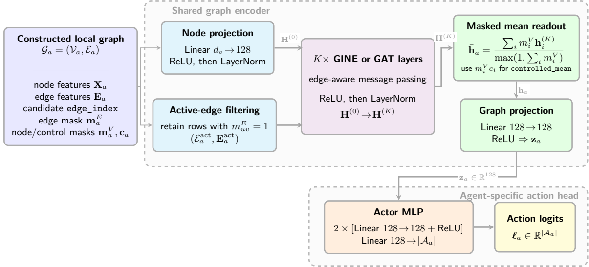
Figure 5.6: End-to-end graph-actor architecture. Candidate edges masked by the current topology are removed before message passing. The graph encoder and its output projection are shared across agents, whereas the final MLP has one output per action available to agent a and is therefore agent-specific.
