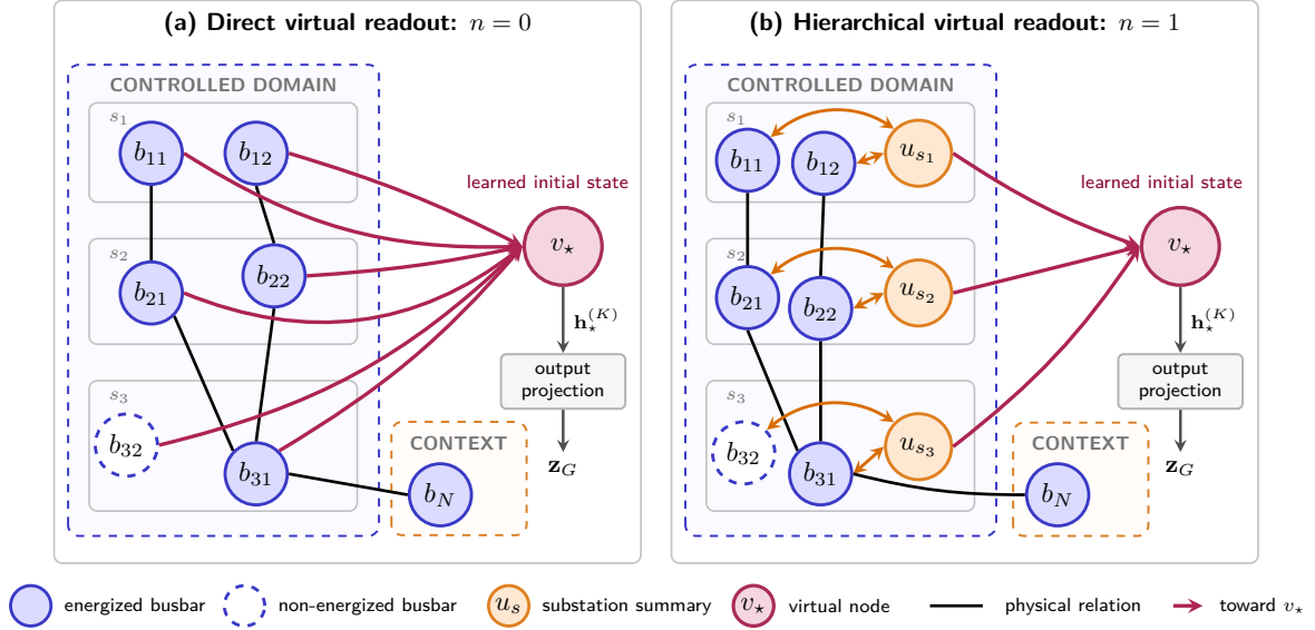
Figure 5.9: Virtual-node readout in the reported one-way setting. Without substation nodes, every controlled busbar—including non-energized b_{32} —sends directly to v_\star . With augmentation n , the same busbars communicate through u_s , and only the substation nodes send to v_\star . The final state \mathbf{h}_\star^{(K)} replaces terminal pooling.
