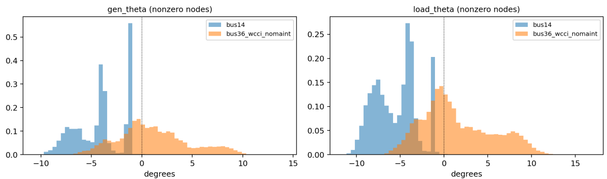
Figure 7.3: Voltage angles at nodes carrying the corresponding asset. The bus14 distributions lie almost entirely on the negative side.
