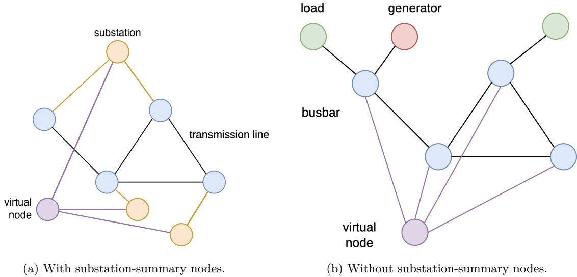
Figure 3.7: Virtual-node graph readout, shown for both definitions of the summary set \mathcal{V}_{\text{sum}} in Equation 3.22. The purple node aggregates that set and its final embedding replaces terminal node pooling. Every purple edge is directed toward the virtual node, which sends no message back. In (a) the substation-summary augmentation of Section 3.3.2 is enabled, so the virtual node attaches to the orange substation nodes and reaches the busbars only through them, which gives a two-level hierarchy busbar \rightarrow substation \rightarrow virtual node. In (b) the augmentation is disabled and the virtual node attaches directly to every included busbar. In neither case does it connect to generator, load, or transmission-line nodes.
