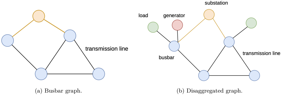
Figure 3.6: Learned substation-summary augmentation, shown in the two schemas of Section 3.2. The orange substation node receives messages from each of its blue busbar nodes and redistributes the resulting substation-level representation through the reverse edges. In (a) the generator and load quantities are aggregated into the busbar features, whereas in (b) they are separate nodes; in both cases the summary node attaches only to busbars, so generators, loads, and transmission-line nodes reach it through their busbar attachments.
