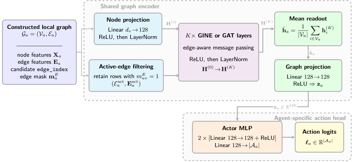
Figure 3.4: End-to-end graph-actor architecture. Candidate edges masked by the current topology are removed before message passing. The graph encoder and its output projection are shared across agents, whereas the final MLP has one output per action available to agent a and is therefore agent-specific.
