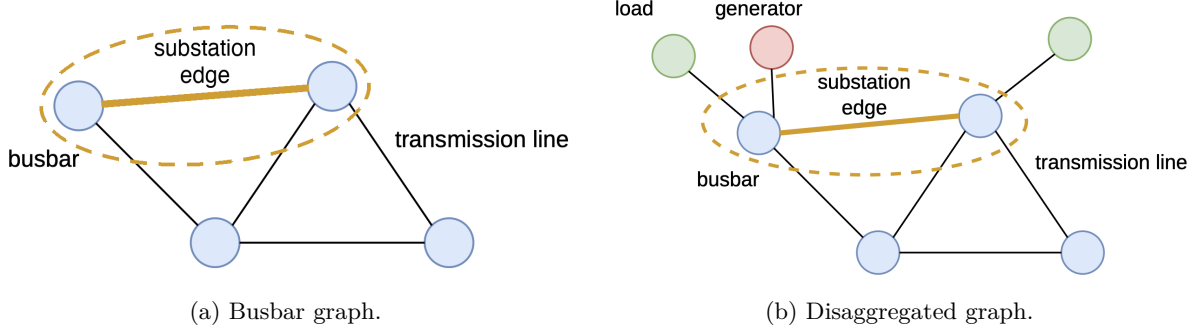
Figure 3.5: Direct same-substation busbar relation, shown in the two schemas of Section 3.2. The highlighted orange edge allows two busbars belonging to the same substation to exchange messages; it is a computational relation and not a physical transmission line. In (a) the generator and load quantities are aggregated into the busbar features, whereas in (b) they are separate nodes. The relation is identical in both cases: it connects two busbars of one substation and does not depend on the node types attached to them.
