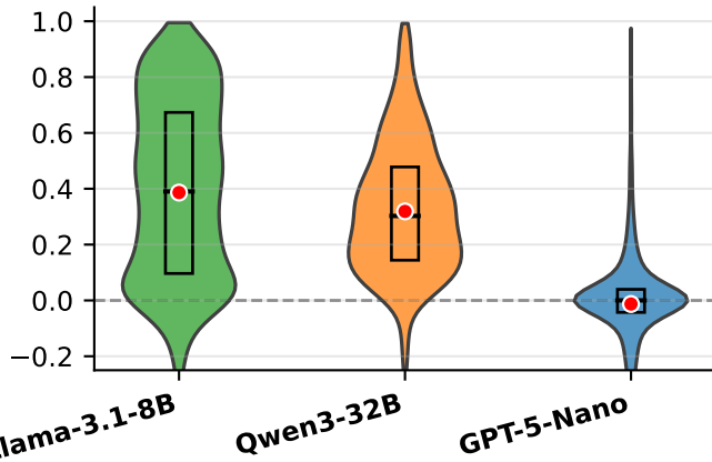
Similarity
