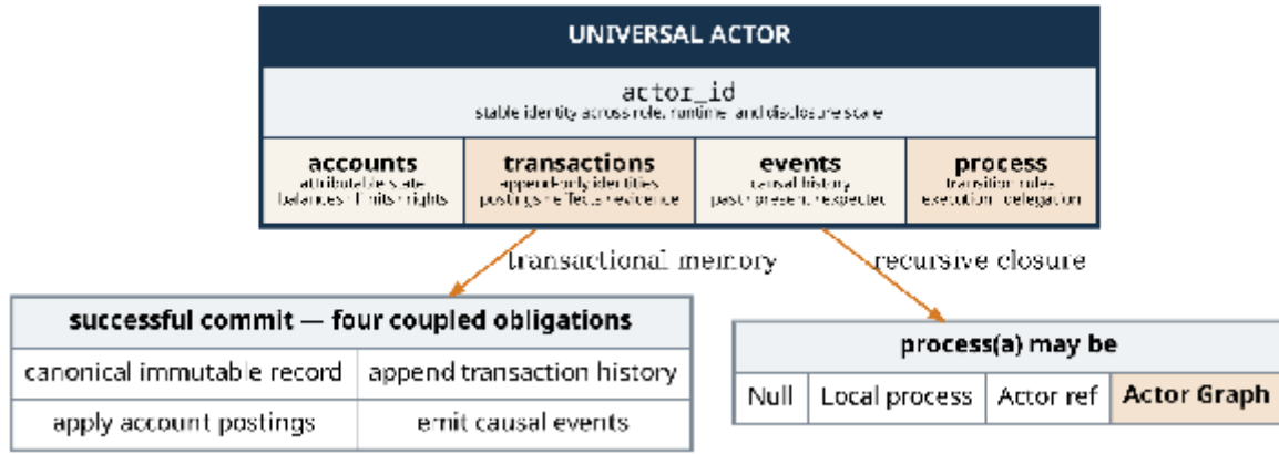
Figure 5: Canonical actor anatomy. Identity, accounts, transactions, events, and process form one operational actor. The commit strip shows all four coupled obligations: preserve a canonical immutable record, append transaction history, apply account postings, and emit causal events; the process may itself reference another Actor Graph.
