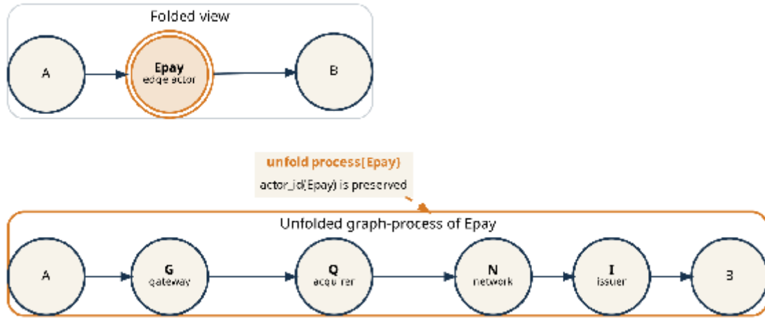
Figure 8: Identity-preserving disclosure of an edge actor. The payment-request path is gateway \rightarrow acquirer \rightarrow network \rightarrow issuer, while \text{actor\_id}(\text{Epay}) remains the outer identity.
