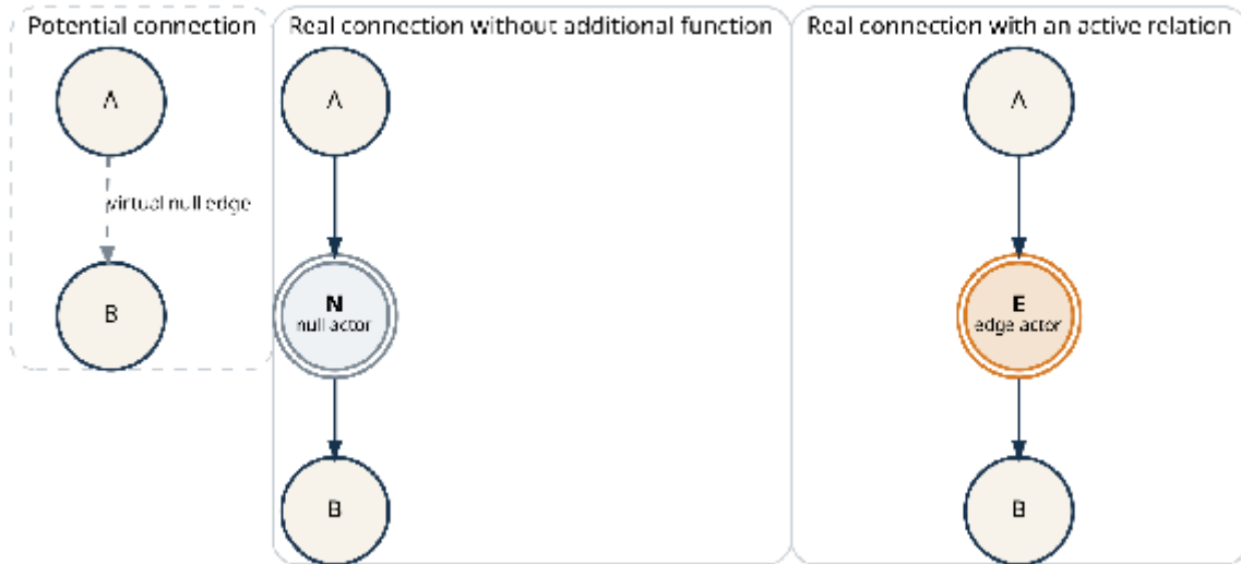
Figure 7: Potential, realised null, and realised functional actor edges.
