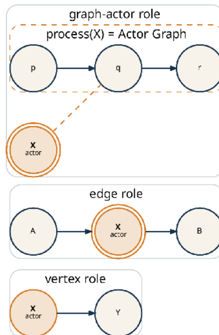
Figure 3: One universal actor type occupying vertex, edge, and graph-actor roles.
