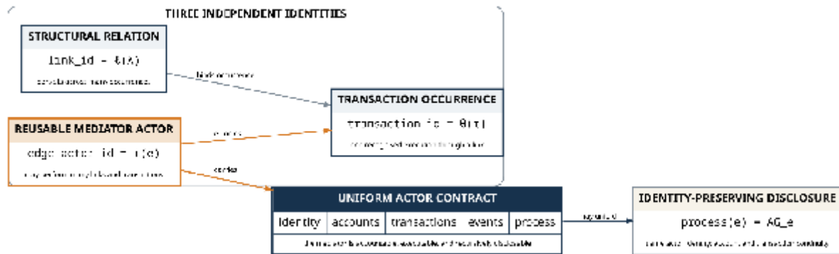
Figure 1: Triple-identity accountable mediation. link\_id identifies the structural relation, transaction\_id identifies one occurrence, and edge\_actor\_id identifies the reusable accountable mediator.
