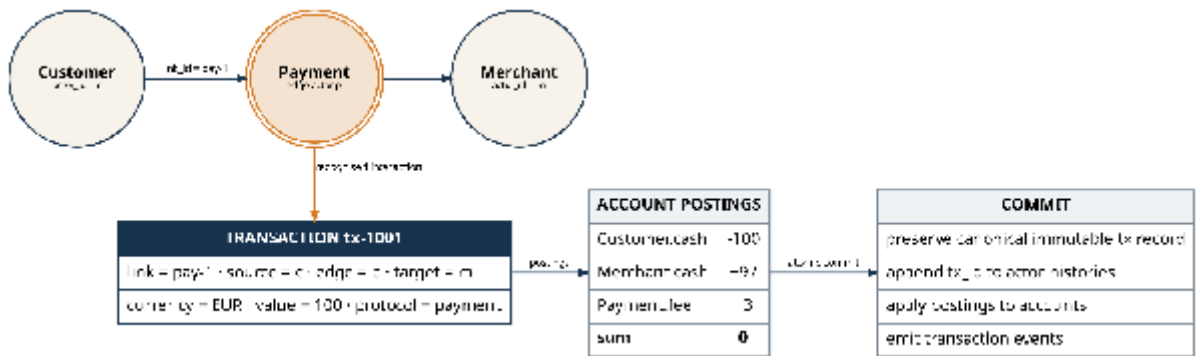
Figure 6: Accounts and transactions are coupled at commit: the transaction is bound to the link and edge actor; its canonical immutable record is preserved, histories append the transaction identity, postings update actor accounts, and transaction events preserve causal evidence.
