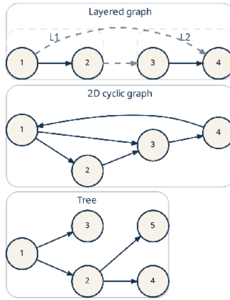
Vertex projections \pi_V(G) — edge actors and link nodes suppressed
