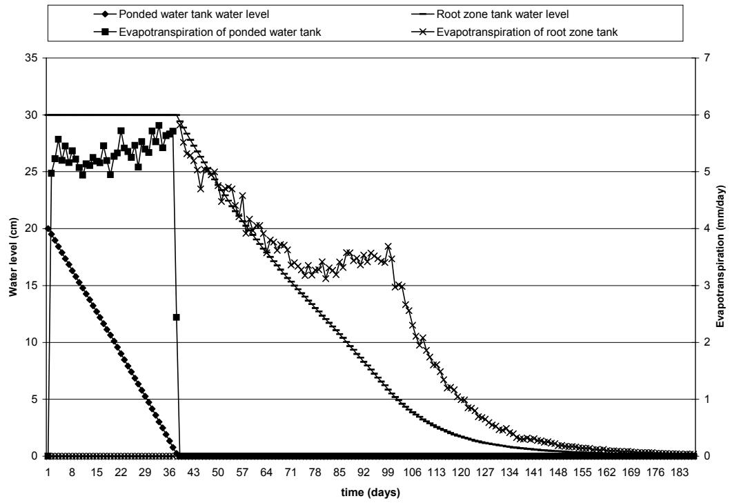
Figure 8. Verification of the evapotranspiration function at the simulated field level.
