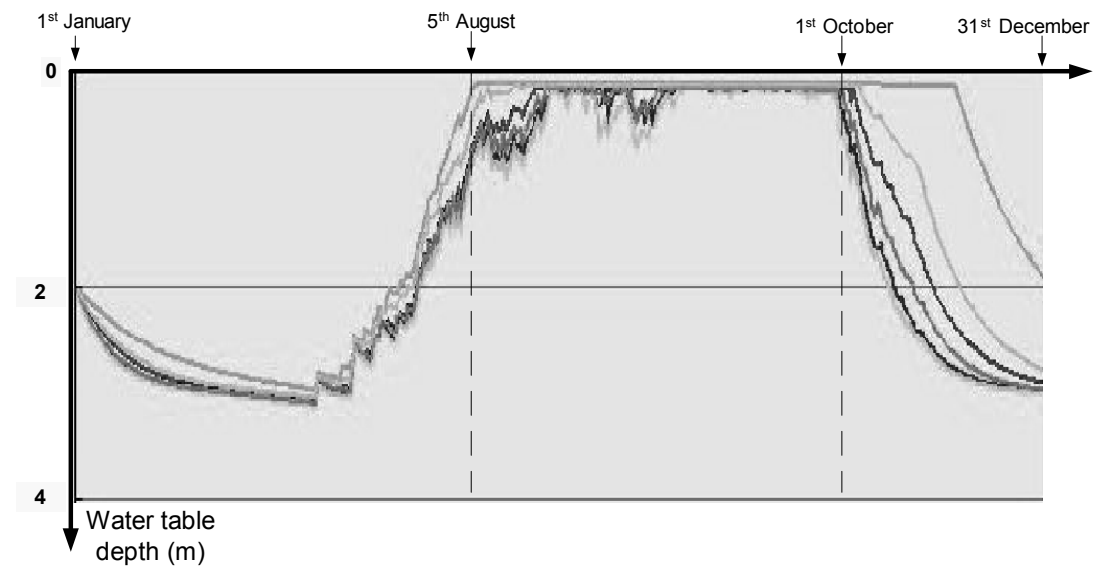
Figure 9. Calibration of the water levels in the six water table tanks of the model. (The six curves represent the water level in each water table tank).
