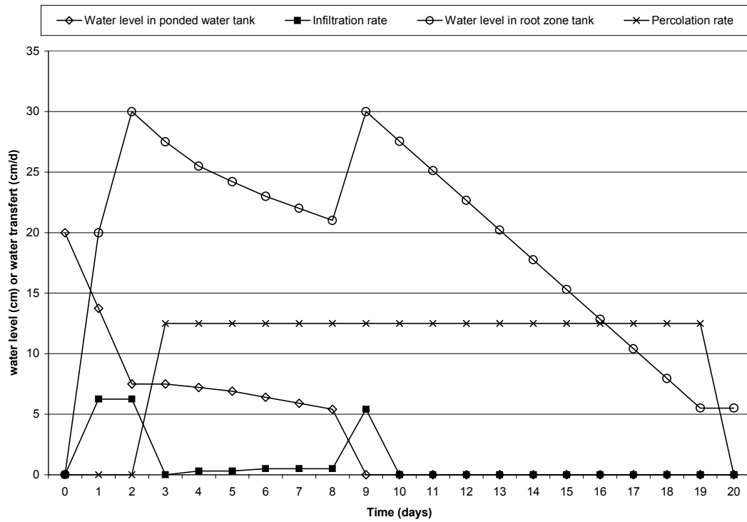
Figure 7. Verification of infiltration and percolation functions in a simulated field.
