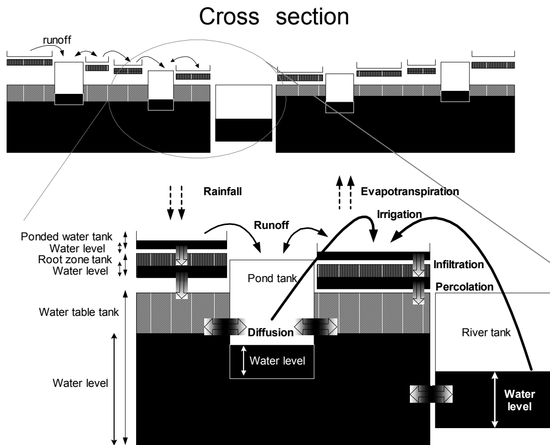
Figure 4. Structure and hydraulic functioning of the multi-agent model.
