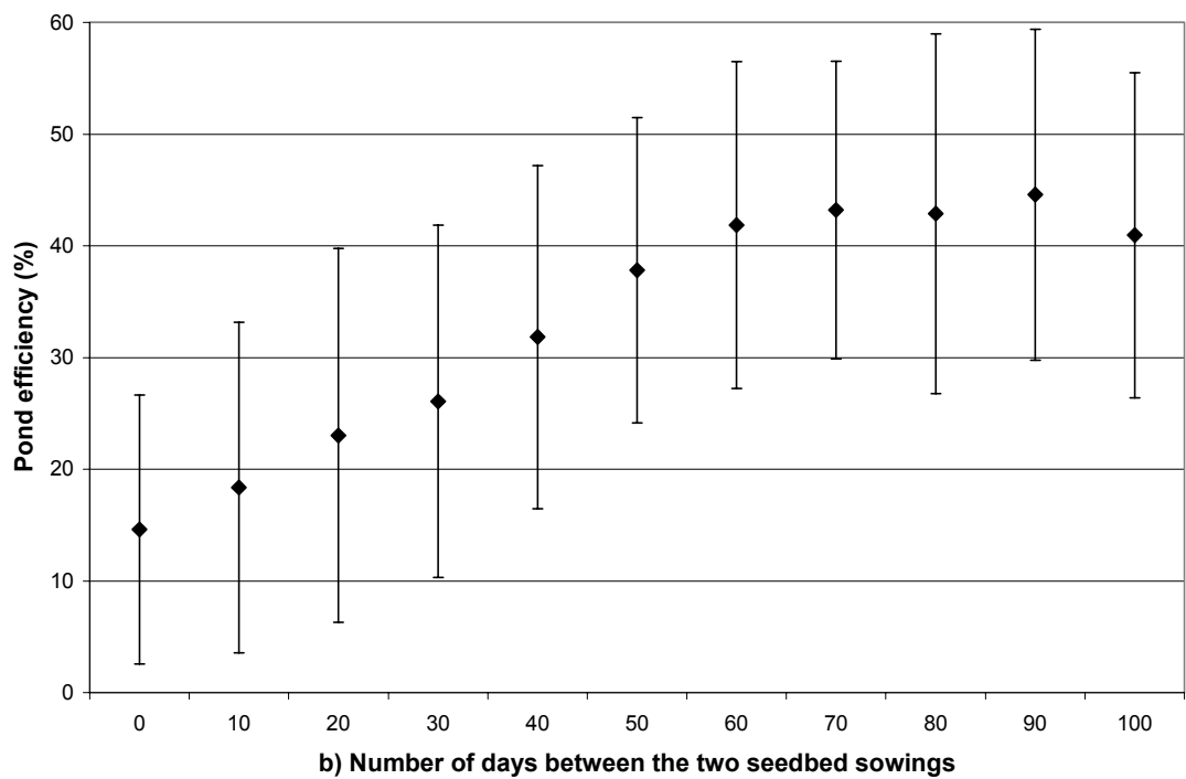
Figure 10. Sensibility analysis of pond efficiency according to variations in the proportion of early sowing of seedbeds (a) and the duration between the two nursery seeding periods (b).
