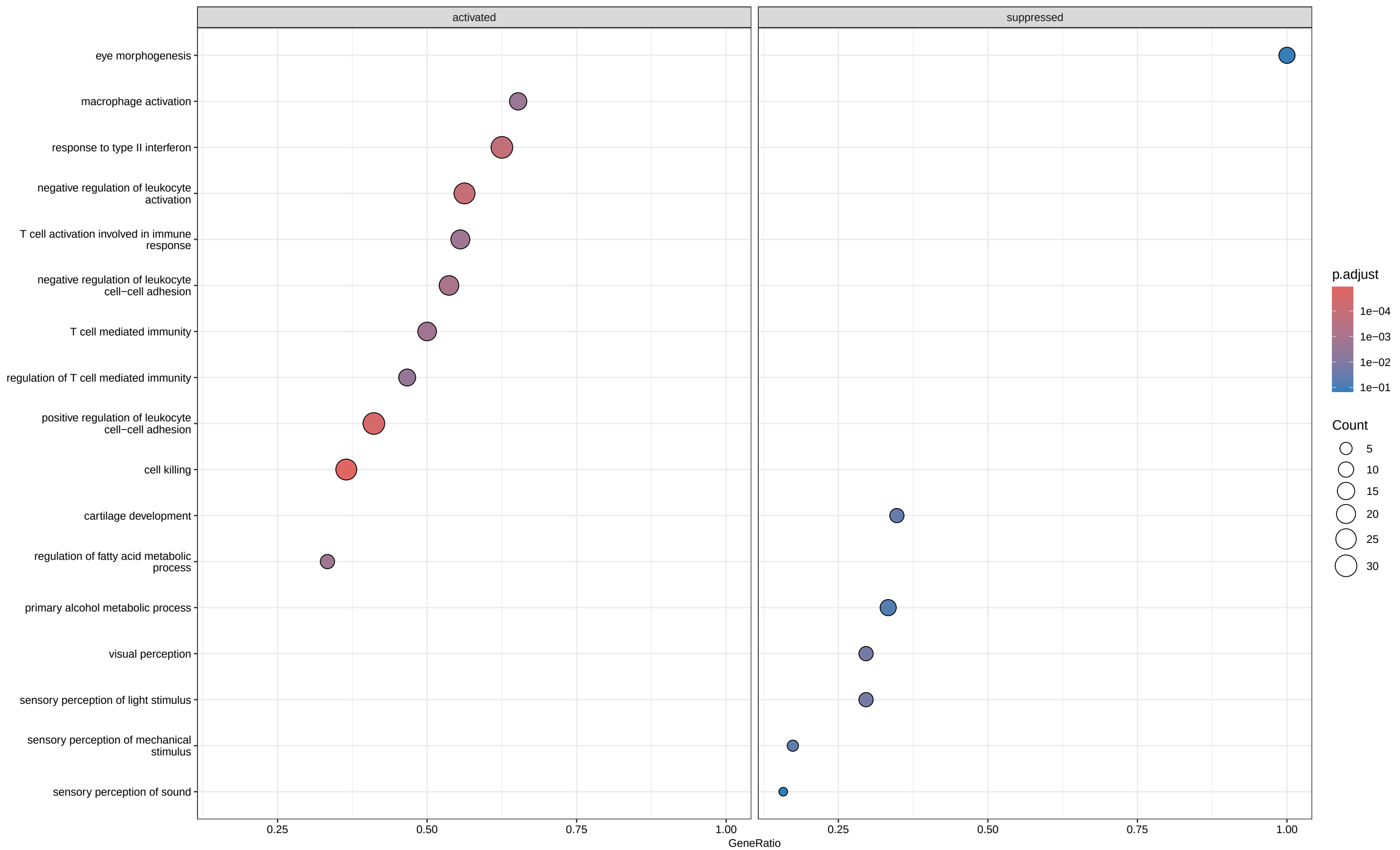
FC vs Healthy: GSEA GO BP top pathways
